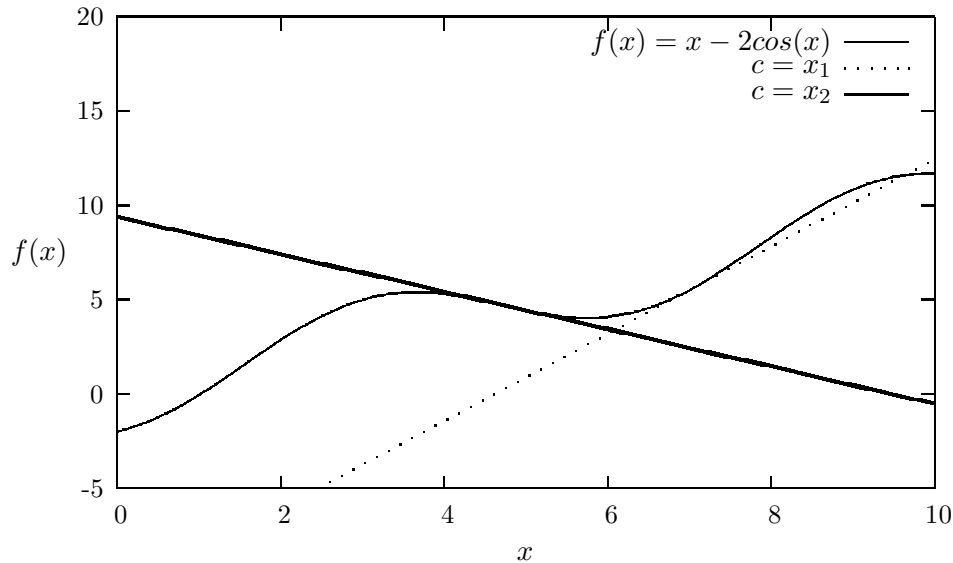
Figure 5.2: Example of a case where Newton-Raphson’s method does not converge. For the function f(x) = x - 2\cos(x) , we see that if we start at x = 7 , the first iteration gives us that the first point where we cross the x -axis is given by x_1 . However, using x_1 as a starting point for the next iteration results in a point x_2 which is close to a local minimum. The tangent here is close to zero and we will never approach the point where f(x) = 0 .
