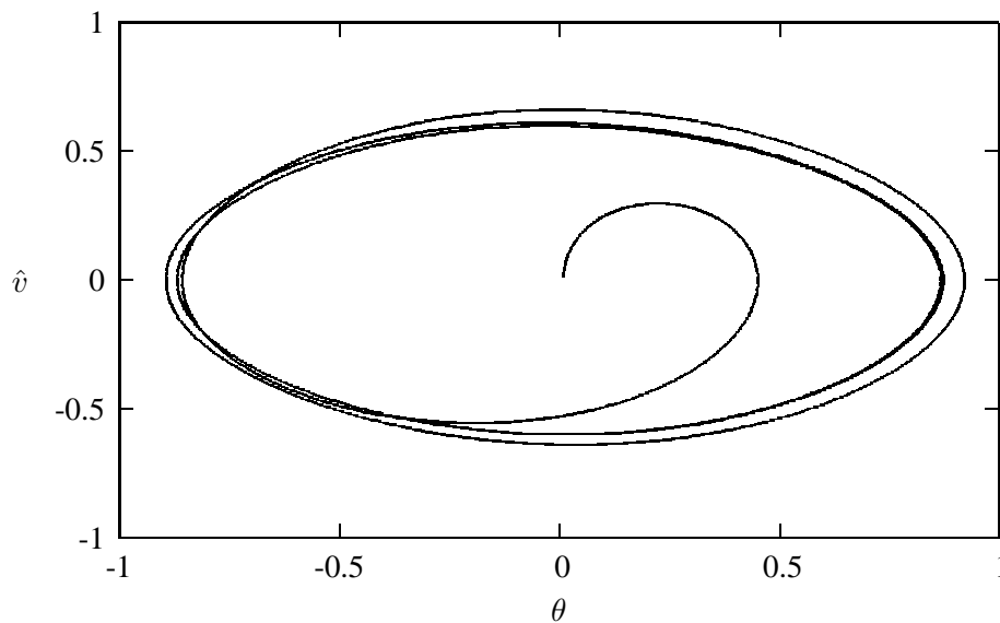
Figure 13.7: Phase-space curve of a linear damped pendulum with Q = 2 , \hat{\omega} = 2/3 and \hat{A} = 0.5 . The initial velocity is \dot{\theta}_0 = 0 and \theta_0 = 0.01 .
