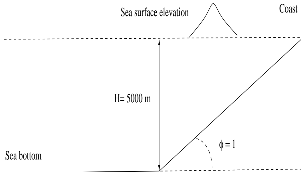
Figure 15.6: The sea bottom towards one of the coastlines has a shape with an inclination of 1 degree. The center of the earthquake is shifted to the right with respect to Fig. 1 as indicated by the exaggerated surface elevation. In this part the surface elevation is moved 40 km to the right.
