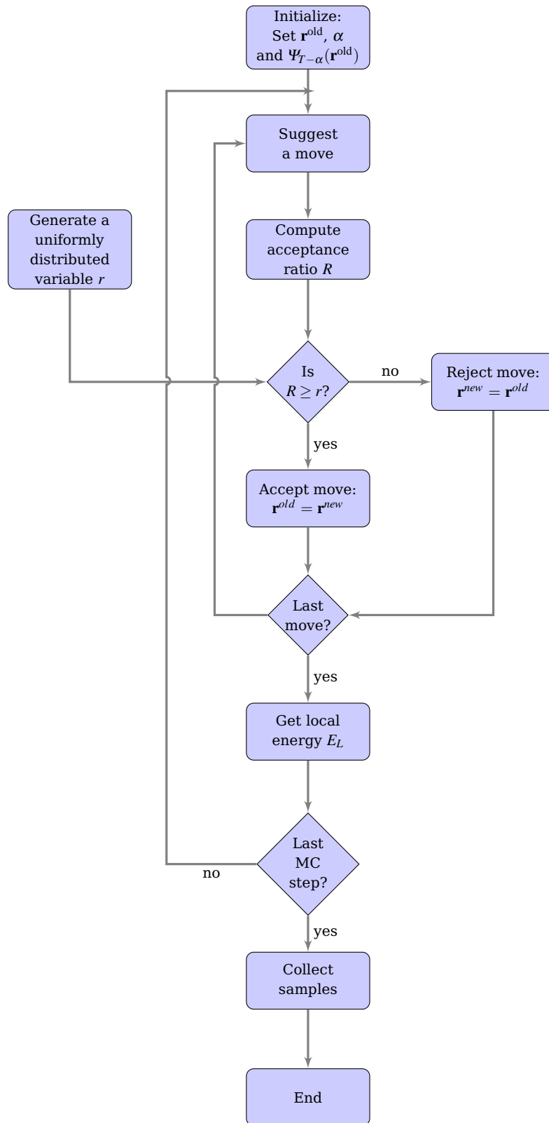
Fig. 14.3 Chart flow for the Quantum Variational Monte Carlo algorithm.
