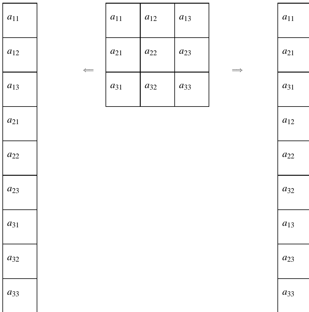
Fig. 6.3 Row-major storage of a matrix to the left (C++ way) and column-major to the right (Fortran way).
