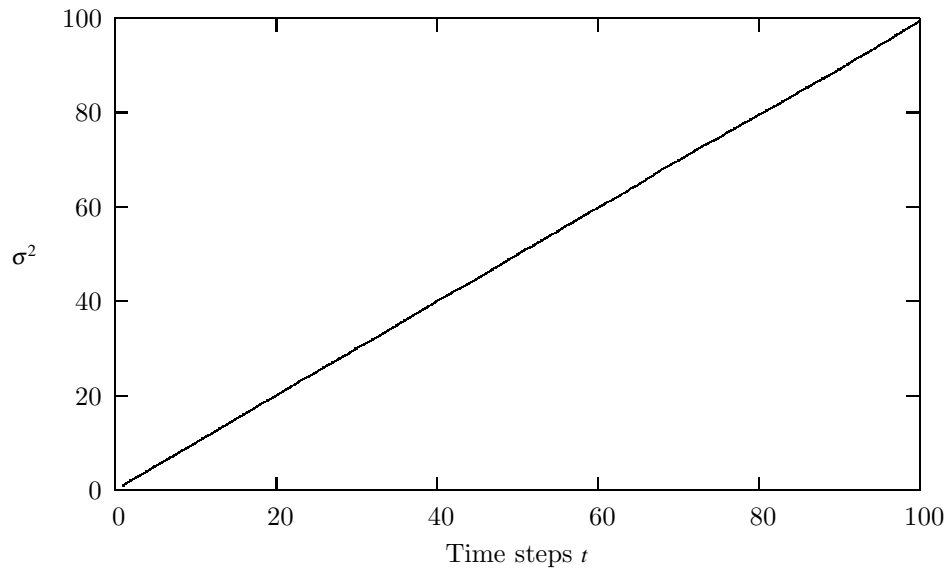
Fig. 12.3 Time development of \sigma^2 for a random walker. 100000 Monte Carlo samples were used with the function ran1 and a seed set to -1 .
