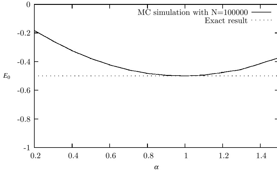
Fig. 14.2 Result for ground state energy of the hydrogen atom as function of the variational parameter \alpha . The exact result is for \alpha = 1 with an energy E = -1/2 . See text for further details.
