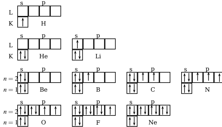
Fig. 15.1 The electronic configurations for the ten first elements. We let an arrow which points upward to represent a state with m_s = 1/2 while an arrow which points downwards has m_s = -1/2 .
