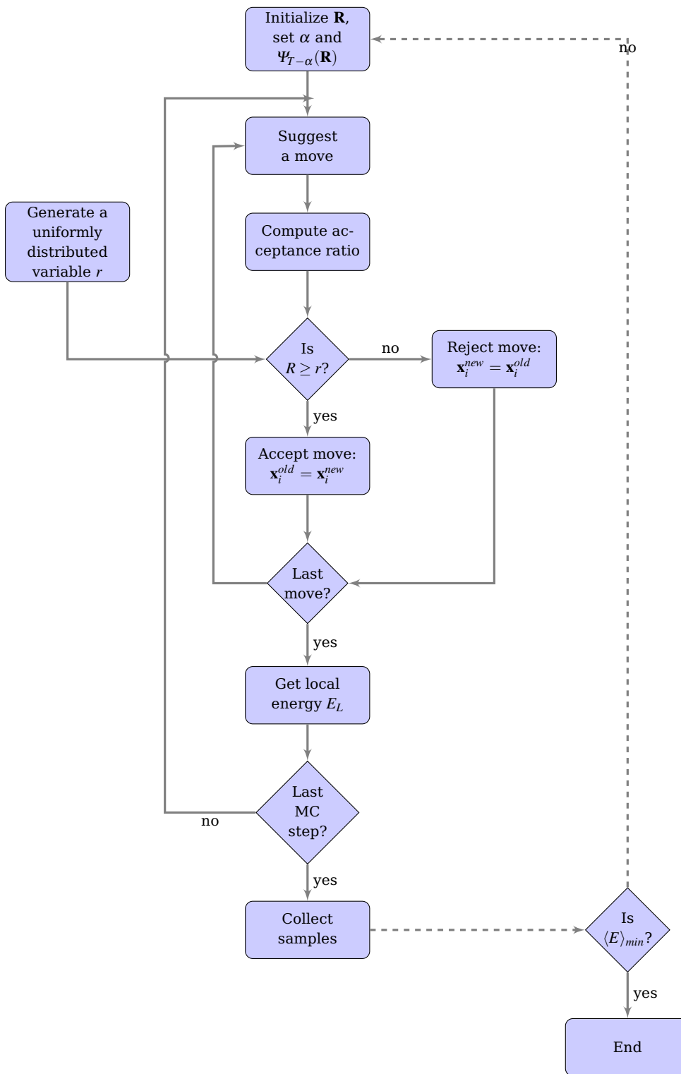
Fig. 16.1 Optimization of the trial wave function \Psi_{trial}(\alpha) and minimization of the energy with respect to the variational parameters.
