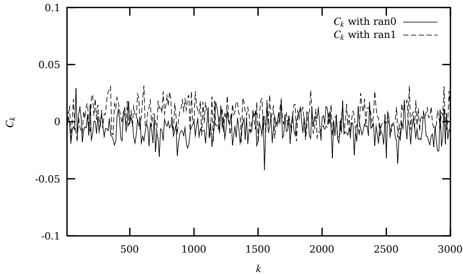
Fig. 11.3 Plot of the auto-correlation function C_k for various k -values for N = 10000 using the random number generators ran0 and ran1 .
