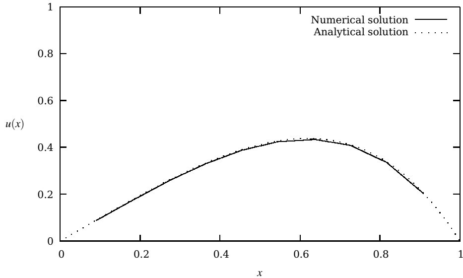
Fig. 6.4 Numerical solution obtained with n = 10 compared with the analytical solution.
