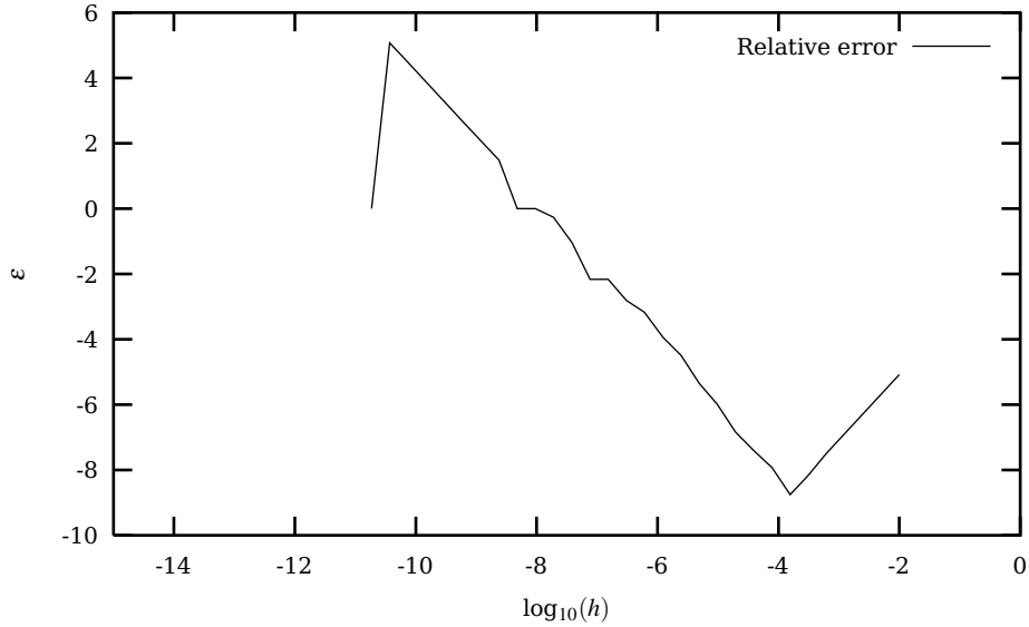
Fig. 3.2 Log-log plot of the relative error of the second derivative of \exp(x) as function of decreasing step lengths h . The second derivative was computed for x = 10 in the program discussed above. See text for further details
