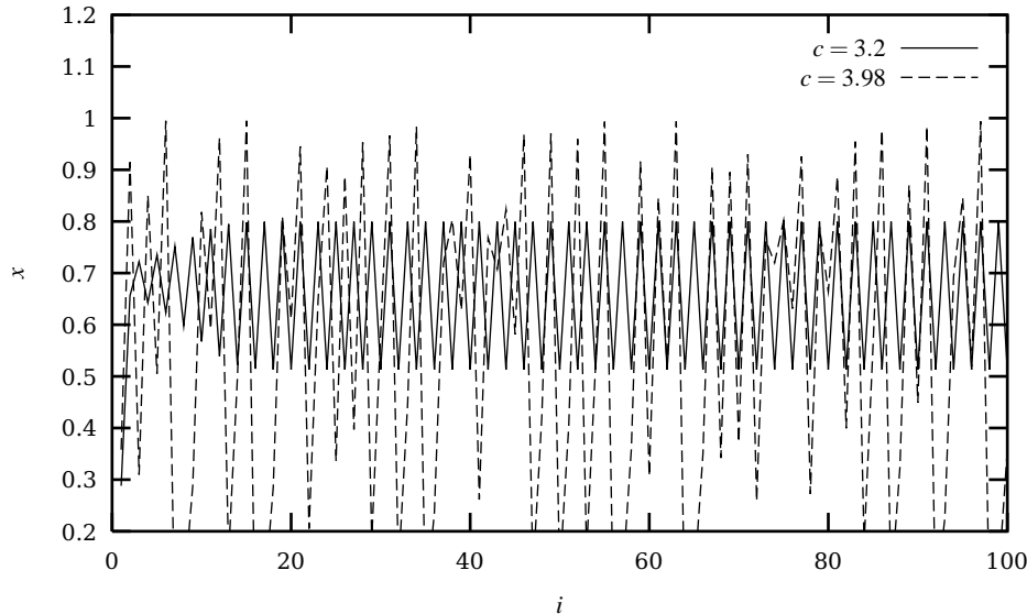
Fig. 11.2 Plot of the logistic mapping x_{i+1} = cx_i(1-x_i) for x_0 = 0.1 and c = 3.2 and c = 3.98 .
