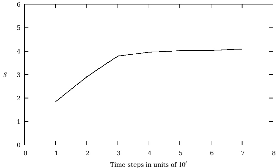
Fig. 12.6 Entropy S_j as function of number of time steps j for a random walk in one dimension. Here we have used 100 walkers on a lattice of length from L = -50 to L = 50 employing periodic boundary conditions meaning that if a walker reaches the point x = L + 1 it is shifted to x = -L and if x = -L it is shifted to x = L .
