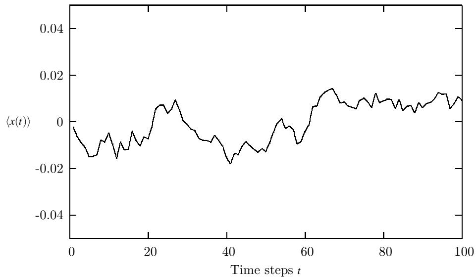
Fig. 12.4 Time development of \langle x(t) \rangle for a random walker. 100000 Monte Carlo samples were used with the function ran1 and a seed set to -1 .
