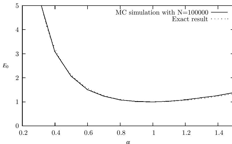
Fig. 14.1 Result for ground state energy of the harmonic oscillator as function of the variational parameter \alpha . The exact result is for \alpha = 1 with an energy E = 1 . See text for further details.
