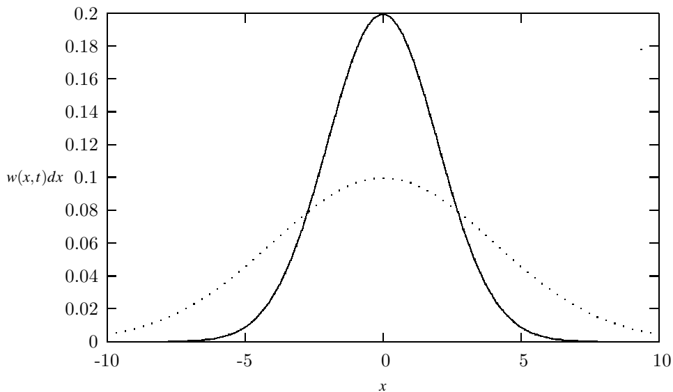
Fig. 12.1 Time development of a normal distribution with variance \sigma^2 = 2Dt and with D = 1\text{m}^2/\text{s} . The solid line represents the distribution at t = 2s while the dotted line stands for t = 8s .
