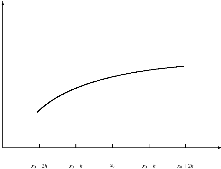
Fig. 3.1 Demonstration of the subdivision of the x -axis into small steps h . Each point corresponds to a set of values x, f(x) . The value of x is incremented by the step length h . If we use the points x_0 and x_0 + h we can draw a straight line and use the slope at this point to determine an approximation to the first derivative. See text for further discussion.
