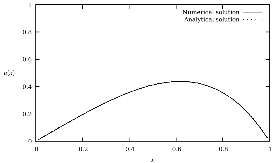
Fig. 6.5 Numerical solution obtained with n = 10 compared with the analytical solution.
