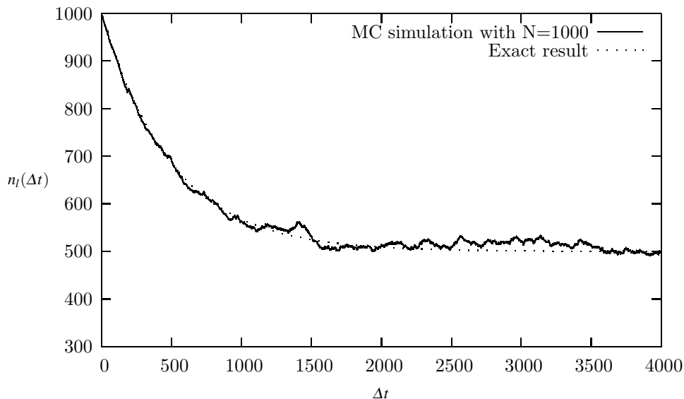
Fig. 11.1 Number of particles in the left half of the container as function of the number of time steps. The solution is compared with the analytic expression. N = 1000 .
