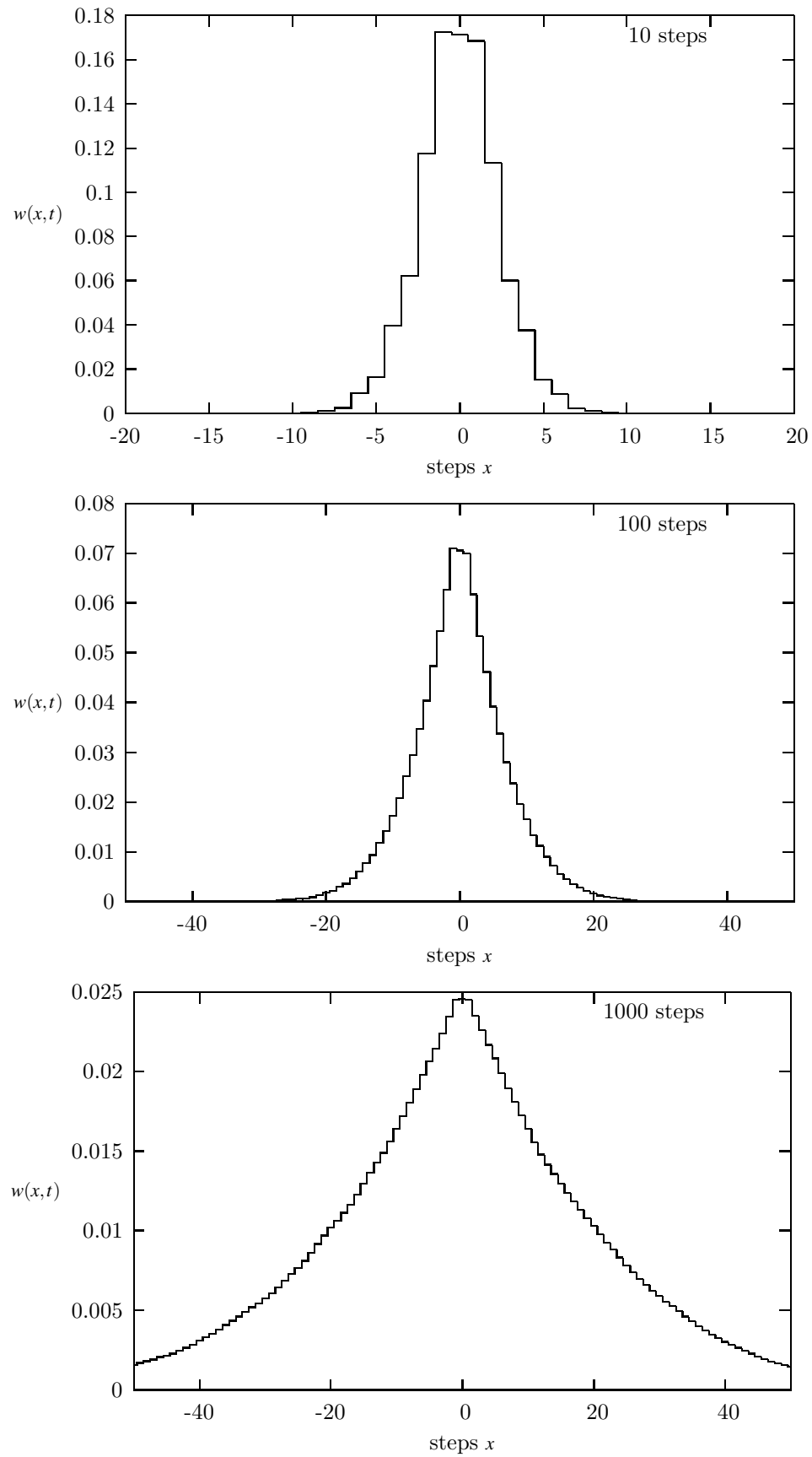
Fig. 12.5 Probability distribution for one walker after 10, 100 and 1000 steps.
