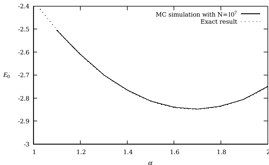
Fig. 14.4 Result for ground state energy of the helium atom using Eq. (14.21) for the trial wave function. A total of 10^7 Monte Carlo moves were used with a step length of 1 Bohr radius. Approximately 50% of all proposed moves were accepted. The variance at the minimum is 1.026, reflecting the fact that we do not have the exact wave function. The variance has a minimum at value of \alpha different from the energy minimum. The numerical results are compared with the exact result E[Z] = Z^2 - 4Z + \frac{5}{8}Z .
