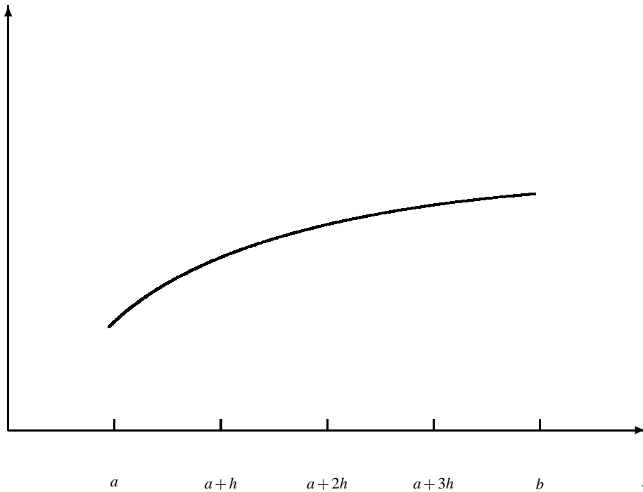
Fig. 5.1 The area enclosed by the function f(x) starting from x = a to x = b . It is subdivided in several smaller areas whose evaluation is to be approximated by the techniques discussed in the text. The areas under the curve can for example be approximated by rectangular boxes or trapezoids.
