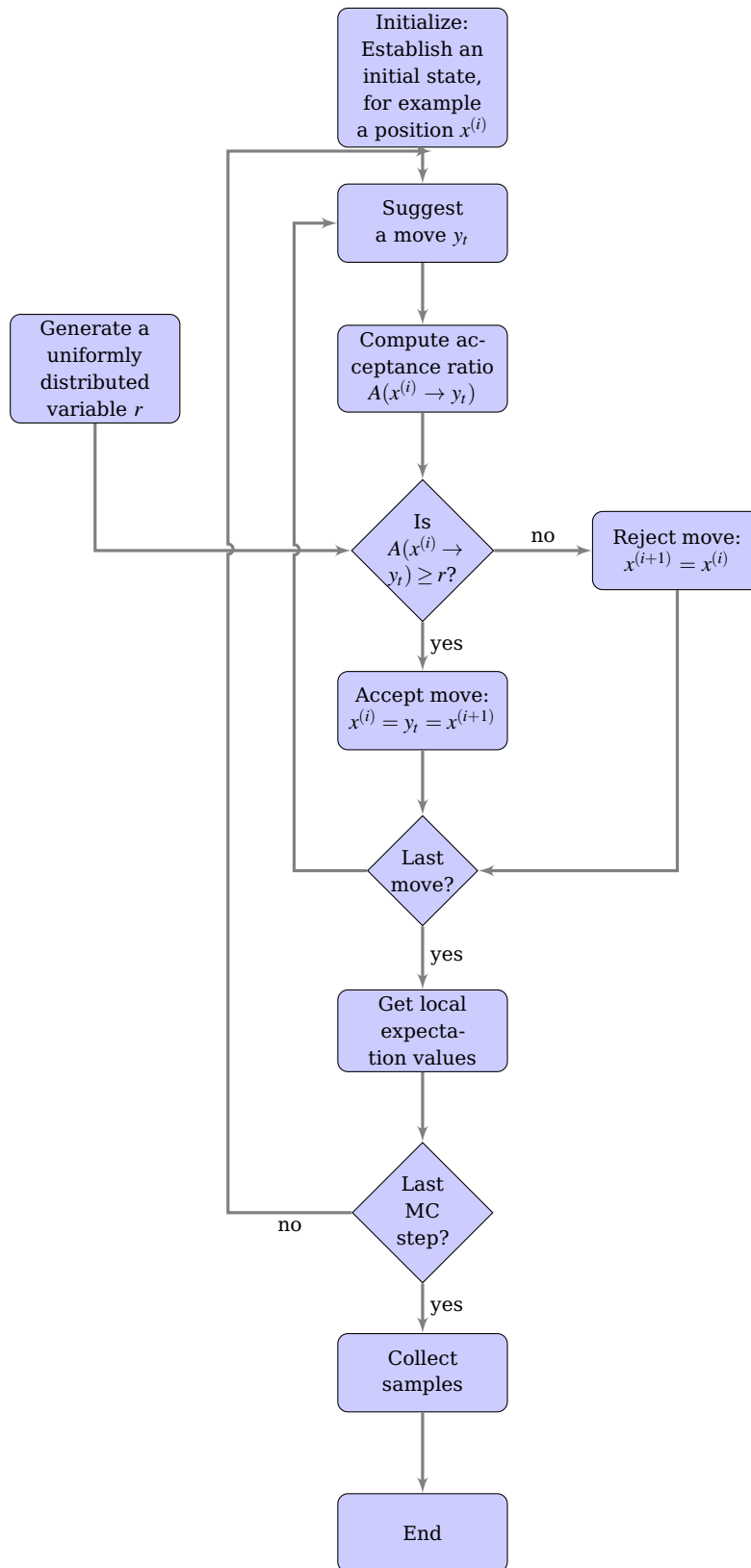
Fig. 12.7 Chart flow for the Metropolis algorithm.
