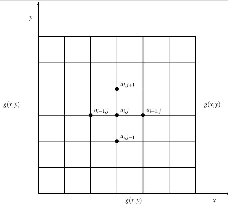
Fig. 10.4 Five-point calculation molecule for the Laplace operator of Eq. (10.14). The border \delta\Omega defines the boundary condition u(x,y) = g(x,y) .
