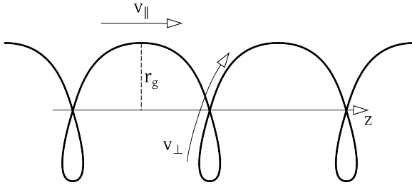
Figure 2: Sketch of the gyromotion for v_{\parallel} \neq 0 .
