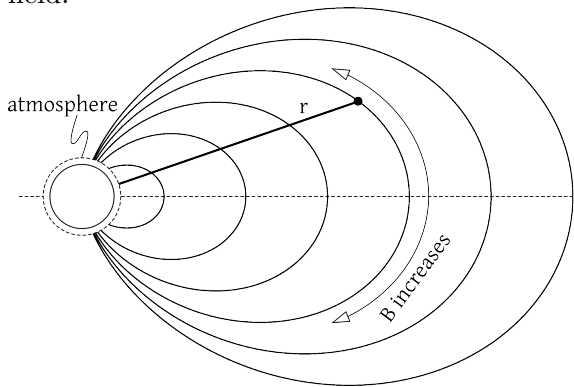
Figure 5: Terrestrial dipolar field lines.
