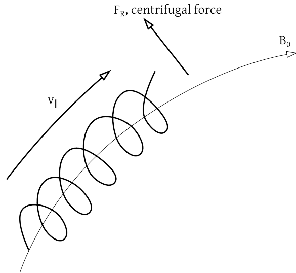
Figure 7: Illustration of the curvature drift. The drift velocity is given by
