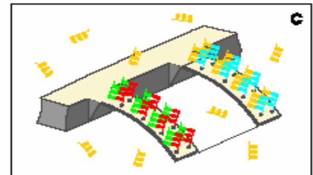
Fig. 2. Scheme illustrating the hybridization experiment. Each cantilever is functionalized on one side with a different oligonucleotide base sequence (red or blue). (A) The differential signal is set to zero. (B) After injection of the first complementary oligonucleotide (green), hybridization occurs on the cantilever that provides the matching sequence (red), increasing the differential signal \Delta x . (C) Injection of the second complementary oligonucleotide (yellow) causes the cantilever functionalized with the second oligonucleotide (blue) to bend.
