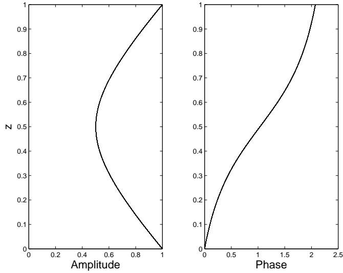
Figure 4.14: The amplitude (left) and phase (right) of the Eady streamfunction vs. height.
