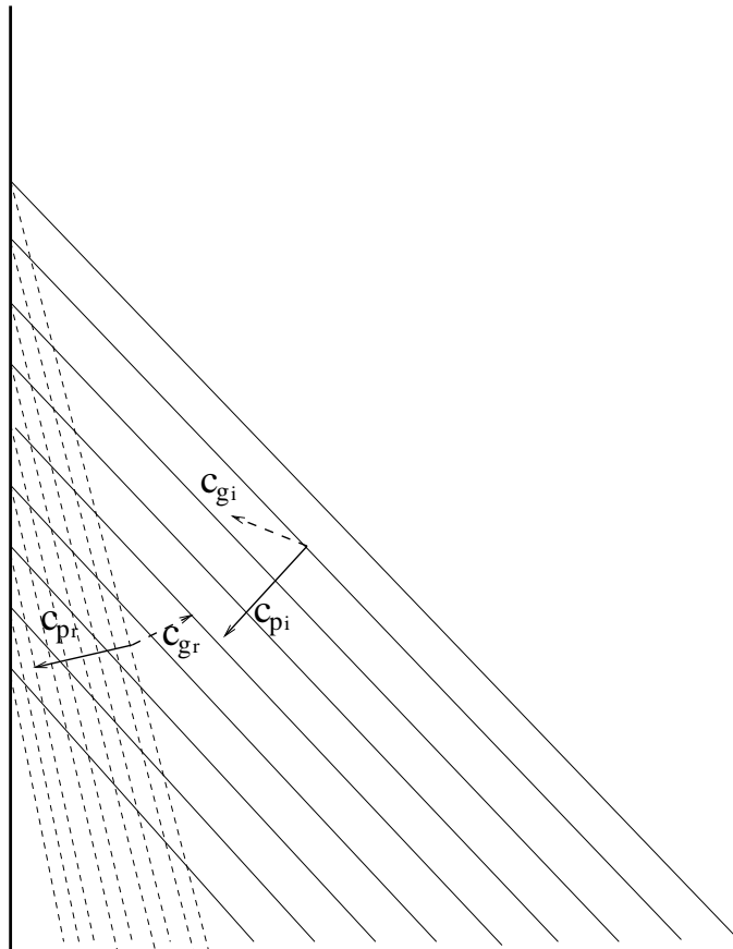
Figure 3.10: A plane Rossby wave reflecting at a western wall. The incident wave is shown by the solid lines and the reflected wave by the dashed lines. The phase velocities are indicated by the solid arrows and the group velocities by the dashed arrows. Note the wavelength in y doesn't change, but the reflected wavelength in x is much shorter. Note too the reflected wave has a phase speed directed toward the wall, but a group velocity away from the wall.
