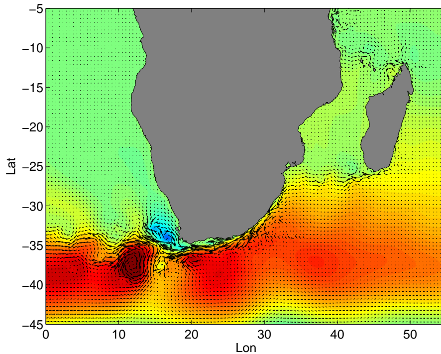
Figure 3.27: The sea surface height from a barotropic numerical simulation of the southern Indian and Atlantic Oceans. From LaCasce and Isachsen (2007).
