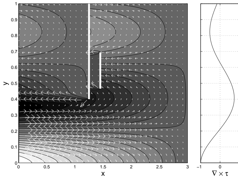
Figure 3.25: A Stommel-like solution for the Indian Ocean. The curl of the wind stress is indicated in the right panel. From LaCasce and Isachsen (2007).
