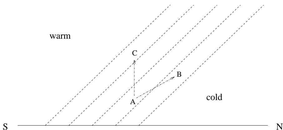
Figure 4.9: Slantwise convection. The slanted isotherms are accompanied by a thermal wind shear. The parcel A is colder, and thus heavier, than parcel C, implying static stability. But A is lighter than B. So A and B can be interchanged, releasing potential energy.
