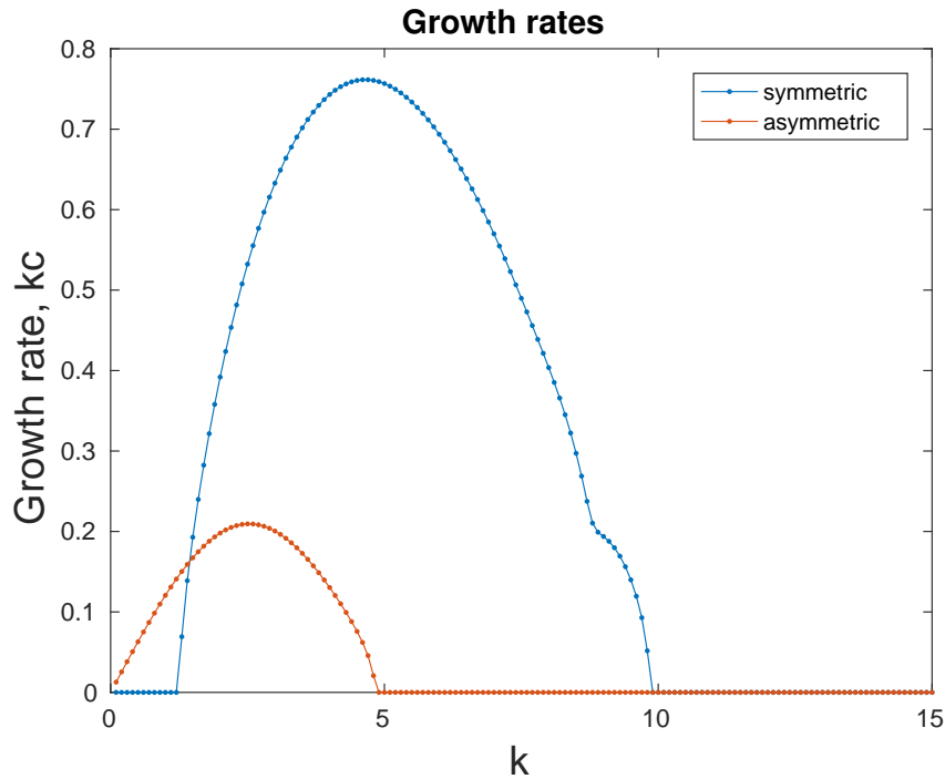
Figure 3.21: The growth rates, kc_i , for symmetric and asymmetric modes, for an eastward sech^2 jet with amplitude U_0 = 1 and a width L = 0.2 .
