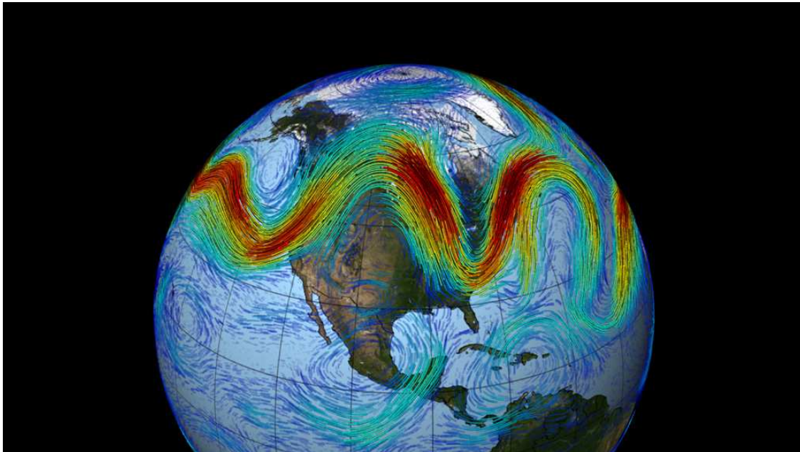
Figure 3.7: An example of Rossby waves in the atmosphere. The Jet Stream, flowing eastward, is superimposed over westward-propagating Rossby waves. Courtesy of NASA.
