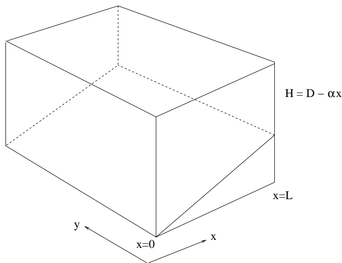
Figure 3.28: A channel with a bottom slope.
