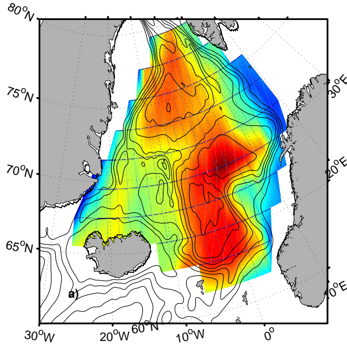
Figure 3.17: Geostrophic contours (solid lines) in the Nordic seas. Superimposed are contours showing the first EOF of sea surface height derived from satellite measurements. The latter shows strong variability localized in regions of closed q_s contours. From Isachsen et al. (2003).
