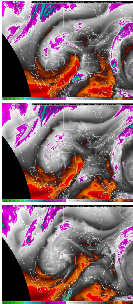
Figure 3.24: Barotropic instability of a filament of dry air, observed from water vapor infrared satellite imagery. The images were taken on the 11th of October, 2005, at 22:45 pm, 3:15 am and 9:45 am, respectively. Courtesy of G. Hakim, Univ. of Washington.
