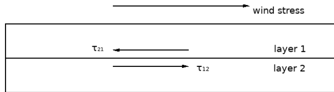
Figure 3.11: The wind acting on an upper layer of fluid at the surface. The layer exerts stress on the layer below, which produces an equal and opposite stress on the upper layer.
