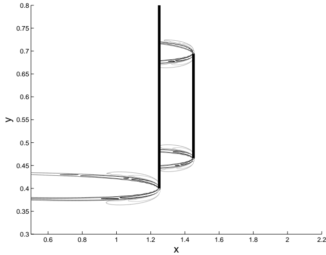
Figure 3.26: The PV gradient for the solution in Fig. (3.25). The gradient changes sign rapidly in the three jet regions. From LaCasce and Isachsen (2007).
