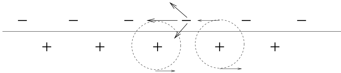
Figure 3.6: The Rossby wave as a string of vorticity anomalies. The cyclone in the right hand circle advects the negative anomaly to the southwest, while the left cyclone advects it toward the northwest. The net effect is westward motion.
