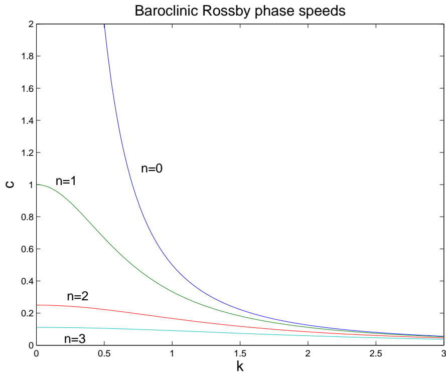
Figure 4.2: Rossby phase speeds as a function of wavenumber for the first four modes.
