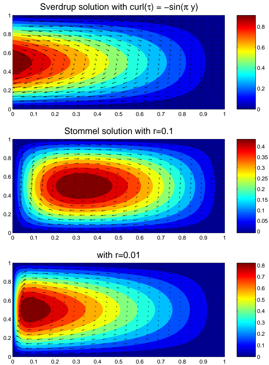
Figure 3.16: Solutions of Stommel's model for two different values of the friction coefficient, r .
