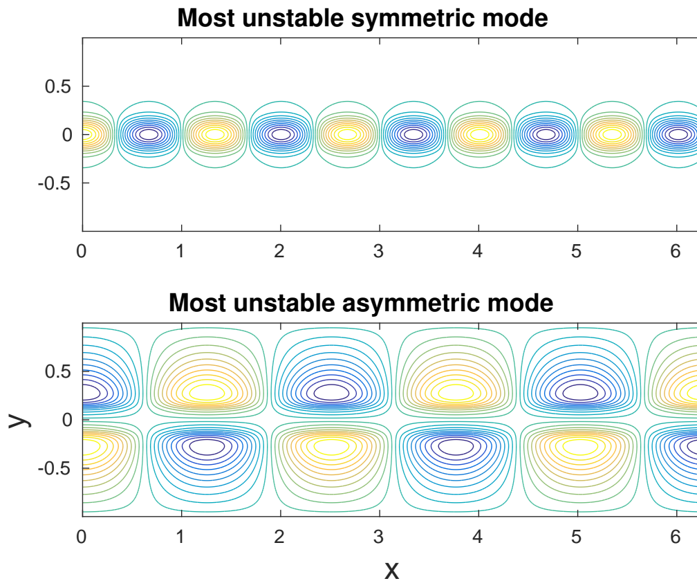
Figure 3.22: The most unstable symmetric and asymmetric waves for the eastward sech^2 jet.
