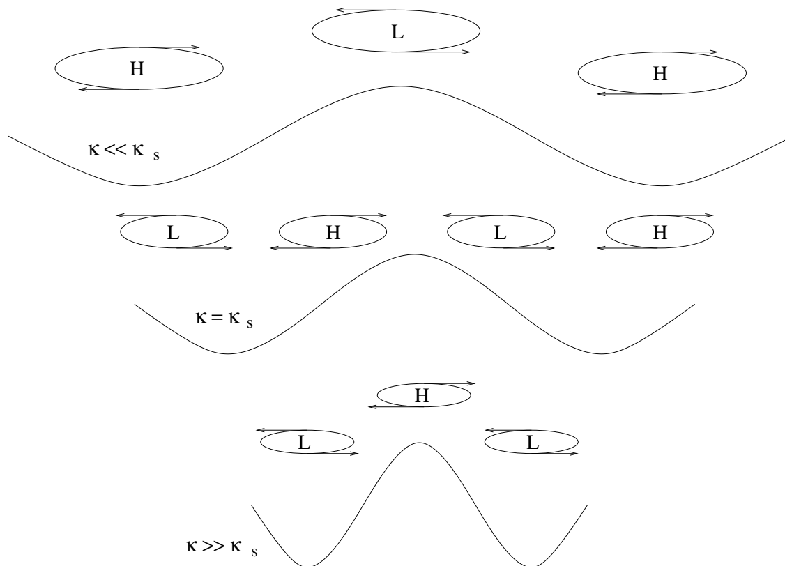
Figure 3.13: The mean pressure distribution over a sinusoidal mountain range. The topographic wavenumber is less than (upper), greater than (bottom) and equal to (middle) the stationary wavenumber.
