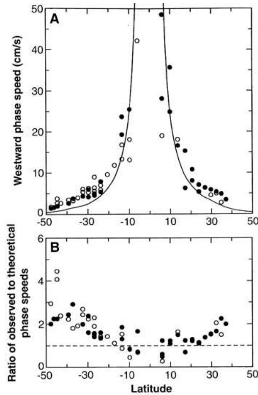
Figure 4.6: Westward phase speeds deduced from the motion of sea surface height anomalies, compared with the value predicted by the long wave phase speed given in (4.43). The lower panel shows the ratio of observed to predicted phase speed. Note the observed speeds are roughly twice as fast at high latitudes. From Chelton and Schlax (1996).
