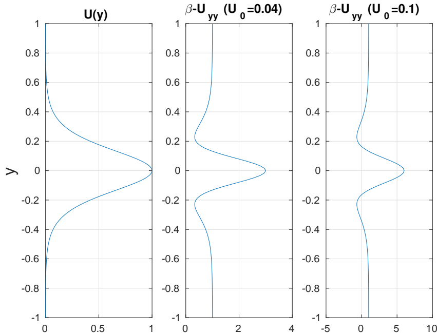
Figure 3.19: An eastward jet (left panel). The middle and right panels show \beta - \frac{\partial^2 u}{\partial y^2} for the jet with amplitudes of 0.04 and 0.1, respectively. Only the latter satisfies Rayleigh's criterion for instability.
