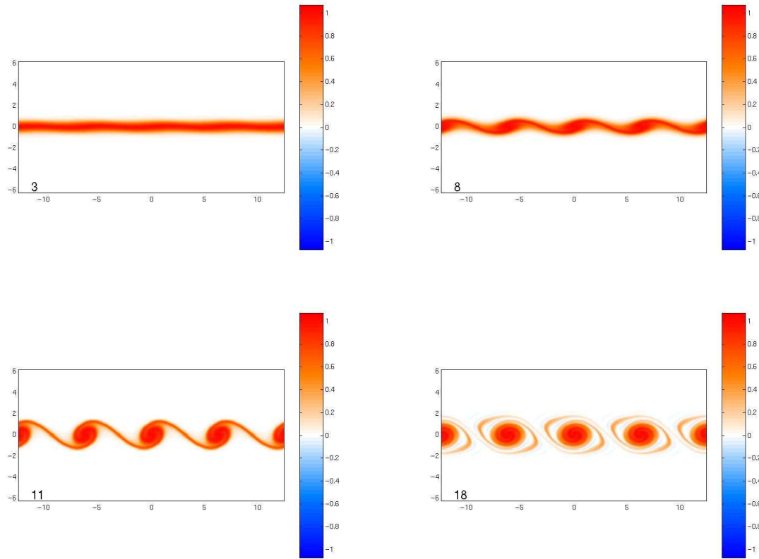
Figure 3.23: Barotropic instability of a jet with a Gaussian profile in relative vorticity. Courtesy of G. Hakim, Univ. of Washington.
