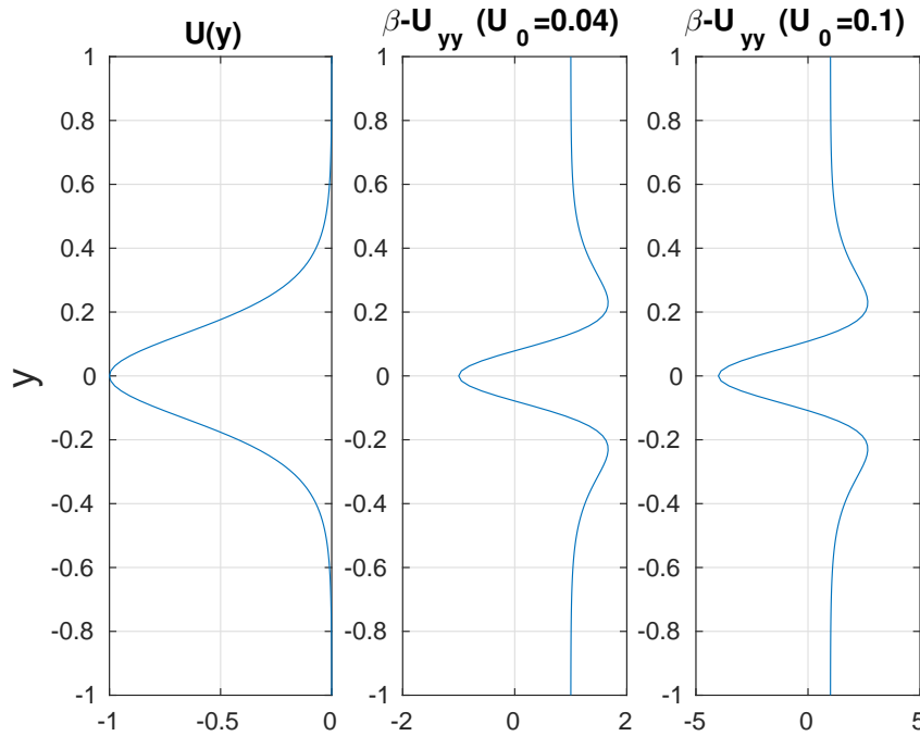
Figure 3.20: A westward jet (left panel). The middle and right panels again show \beta - \frac{\partial^2 u}{\partial y^2} for the jet, with amplitudes of 0.04 and 0.1. Note that both satisfy Rayleigh's criterion for instability.
