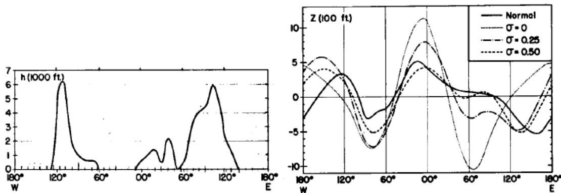
Figure 3.14: Charney and Eliassen's (1949) solution of the barotropic mountain wave problem at 45N. The topographic profile is shown in the left panel (their Fig. 3). The mean pressure at 500 mb is shown in the right panel (their Fig. 4) as the solid line. The dashed lines indicate the theoretical solutions, using three different values of friction.
