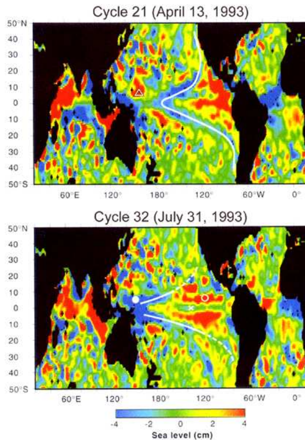
Figure 3.8: Sea surface height anomalies at two successive times. Westward phase propagation is clear at low latitudes, with the largest speeds occurring near the equator. From Chelton and Schlax (1996).
