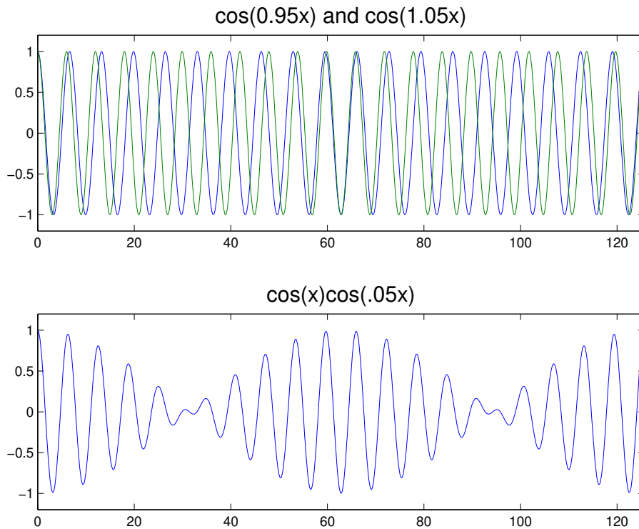
Figure 3.9: Two waves with nearly the same wavelength (upper panel) and their sum (lower panel).
