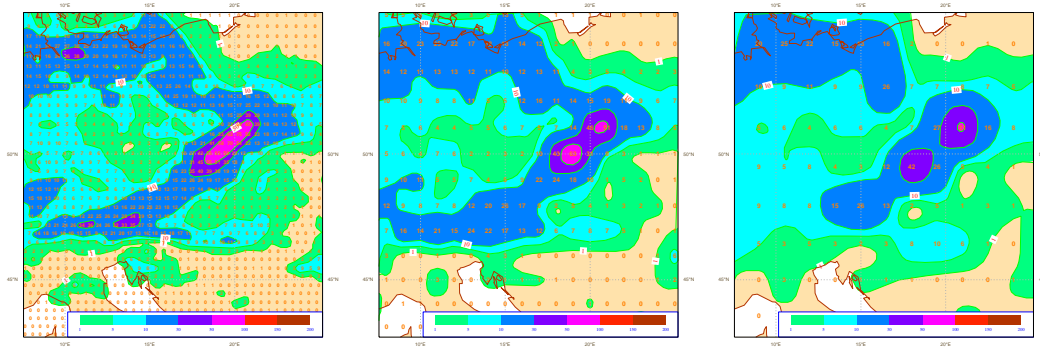
Figure 15 : The impact of interpolation on surface fields. Grid-point values and contours of 24h total precipitation predicted by the T511. From the left to the right: the field on the original gaussian grid at full resolution, the field interpolated over a 1 deg. lat-lon grid and the field interpolated over 1.5 deg. lat-lon grid.
