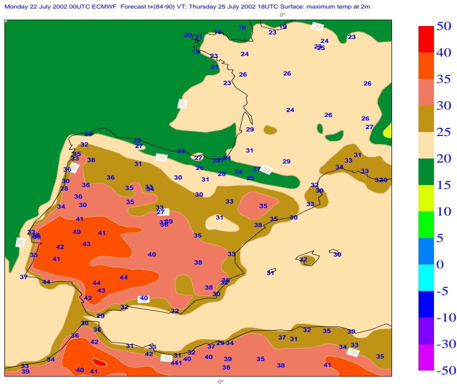
Figure 6 : An example of D+4 forecast of 2m maximum temperature (shaded) compared with observations (numbers) during 2002 heat wave over southern Spain. The model was very skillful in predicting the regions with higher temperatures even if the extreme peaks were underestimated
