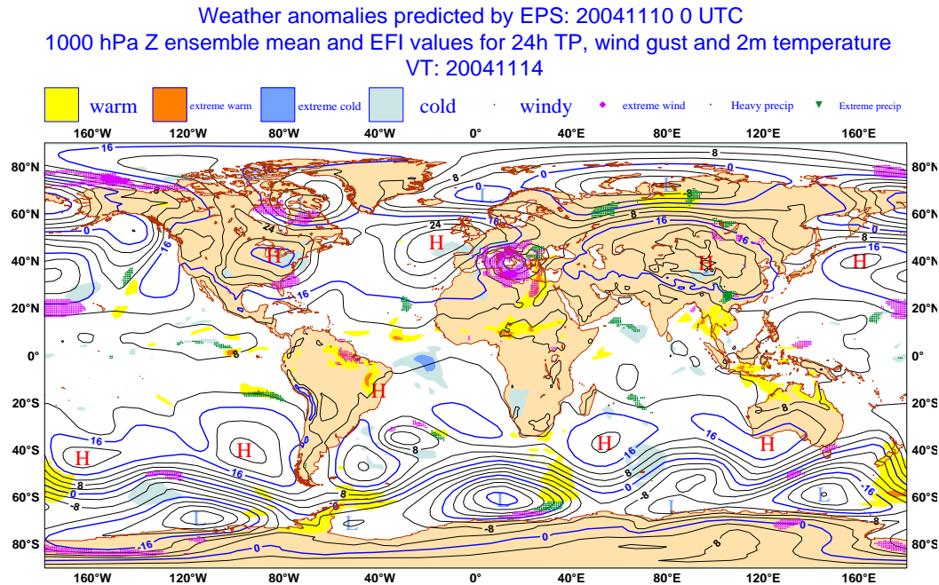
Figure 44 : Weather anomalies map based EFI values and 1000 hPa ensemble mean.
