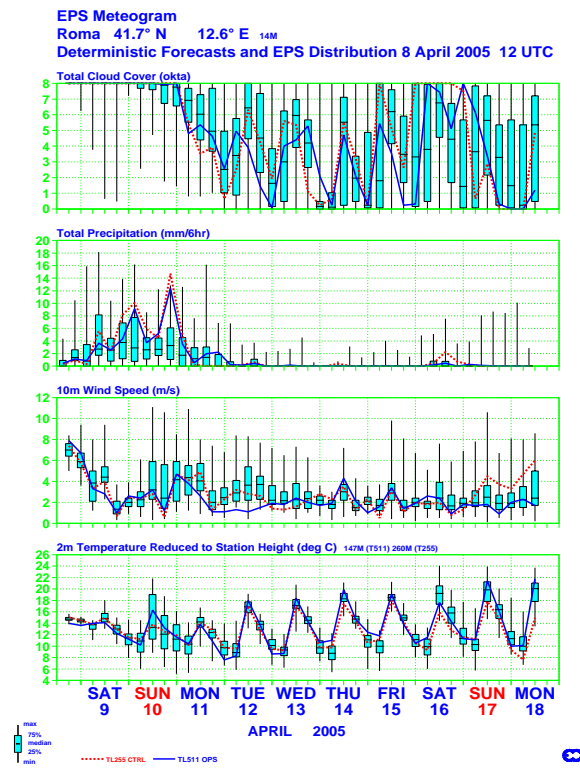
Figure 32 : The forecast uncertainty, as indicated by the EPS spread, is changing with the parameter, it is usually larger for cloud cover, and it usually increases with the forecast step. However uncertainty is also flow or feature dependent and there might be cases, as this EPSgrams example shows, where forecast uncertainty is larger at shorter forecast steps. In this case uncertainty in the positioning of a surface low has resulted in a large spread in wind and precipitation.
