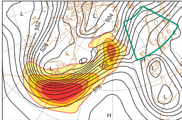
Prediction based on TE-d42 singular vectors
