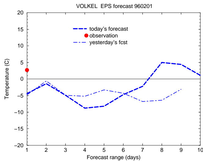
Figure 23 : The forecast 2-meter temperature forecast for Volkel in the Netherlands in winter 1995 according to two consecutive ECMWF forecasts. They are 8° K wrong 24 hours into the forecast and inconsistent during the second half of the period.
