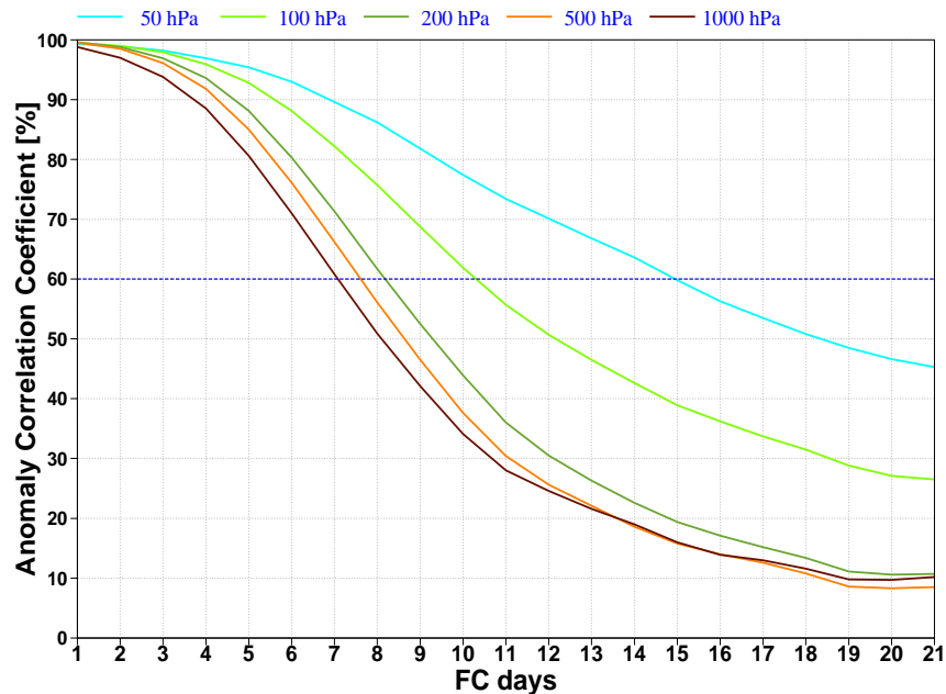
Figure 1 : Anomaly Correlation Coefficient for ECMWF forecasts (EPS Control) for different levels over the Northern Hemisphere in 2004. The skill of the forecasts increase with height. Skilful ten day forecasts has been a reality for the stratosphere for long times.
