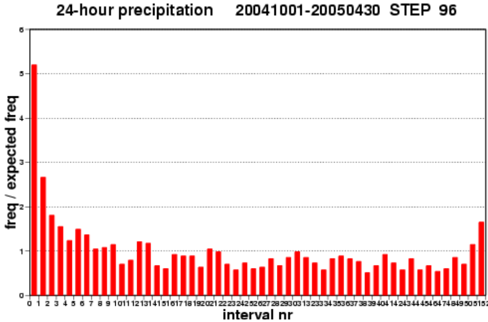
Figure 21 : Example of Talagrand diagram for EPS precipitation forecast over Scandinavia. For every observation point and date all the members are ordered according to their forecast values, from the smallest to biggest. For an EPS with 50 members there are 51 intervals including the unlimited intervals at the edges of the distribution. The y-axis indicates the number of cases (relative to the total number) the analysis is found between two ordered adjacent members on the x-axis. The U-shape indicate that the ensemble does not spread out sufficiently, the tendency to have a J-shape that the system has a wet bias
