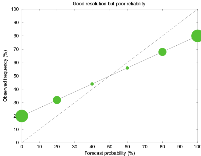
Figure 19 : An example of a typical over-confident probability forecast system. When the system is absolutely sure a certain weather will not occur (0%) or will occur (100%) it is wrong by 20%.
