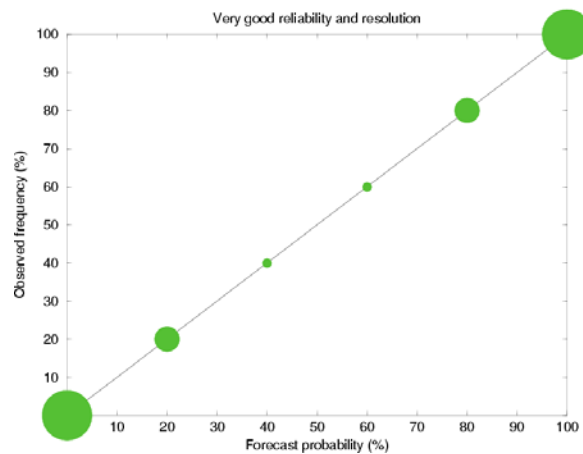
Figure 18 : A schematic example of reliability diagram. The x-axis indicates the forecast in intervals of 20%, the y-axis the observed proportions of occurrences in each probability interval. The size of the filled circles indicate the total number of forecasts for each category. This forecast system is very good with perfect reliability and a majority of forecasts in the high and low probabilities (good resolution).
