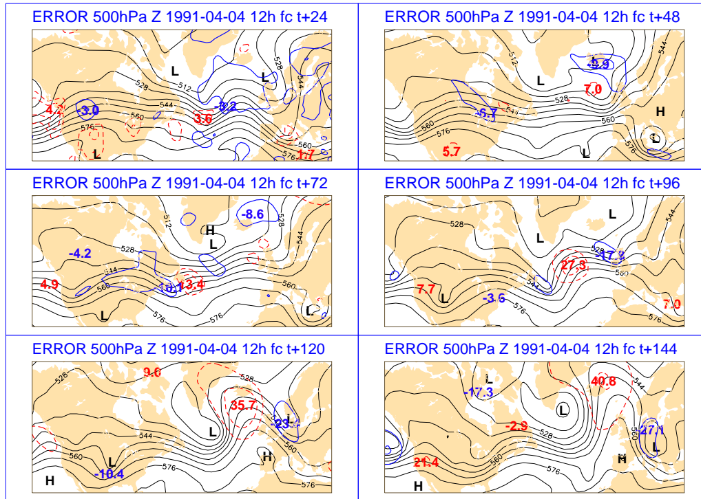
Figure 11 : An example of error tracking. The 500 hPa Z forecast (black lines) and errors (red/positive, blue/negative) from 4 April 1991. A TEMP SHIP on the northwest Pacific had been wrongly decoded and caused a 20-30 gpm positive analysis error (+4.2 dgpm at +12h). Early in the forecast a new negative error (-3.0 dgpm) is created downstream over W USA. While it moves eastward under amplification (amplifying from -6.7 to -18.1 dgpm) another error of opposite sign (amplifying from +13.4 to +27.8 and 35.7) is followed by a fourth error which was associated with a spurious cut-off over NW-Europe.
