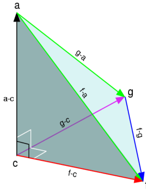
Figure 50 : The case with two realistic, but skill-less forecast systems (f) and (g), can be illustrated by an extension to the concept in figure 48, as a three-dimensional vector diagram. The “consistency” or “jumpiness” is represented by the vector (f-g). By “watching” the geometrical figure from the upper right (facing down to the left) yields the image in figure 51 below
