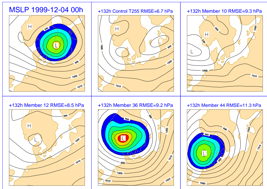
Figure 16 : On 4 December 1999 Denmark was severely hit by an extremely forceful storm. The figure shows the pressure patterns for the verifying analysis at 00 UTC, and five 132 h forecasts (EPS Control and four members, all run at T255). Those two members which actually had the storm, but with a certain phase error, scored worse than those three which had no storm at all.
