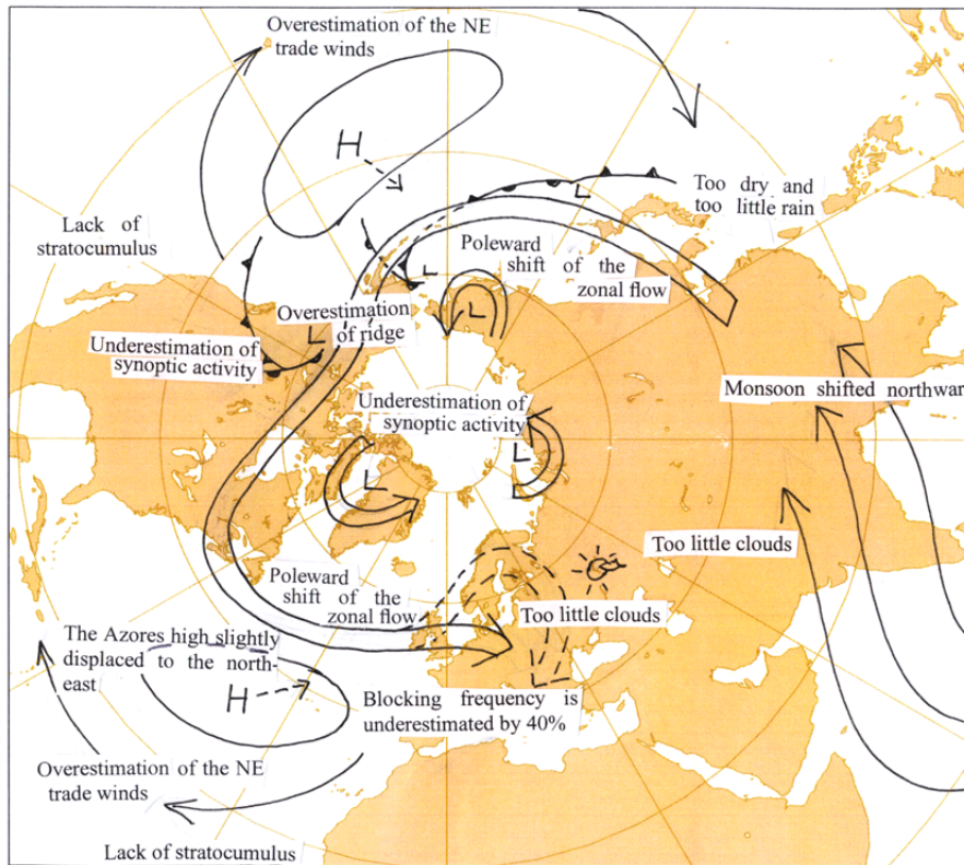
SUMMER: Eddy kinetic energy underestimated on all scales
