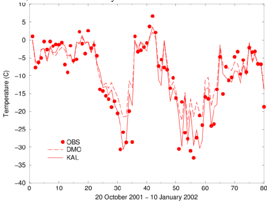
Figure 39 : The statistical interpretation has modified the NWP output mainly for the cold regimes where the systematic error was large.
