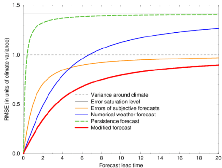
Figure 29 : Same as figure but with the error growth of an ensemble mean forecast included. It incorporates the accuracy of the short range NWP with a convergence toward the errors saturation level of a climate statement. A poor man’s ensemble mean is likely to lie between the red and blue lines, dependent on the number of “ensemble members” and the quality of the deterministic models.
