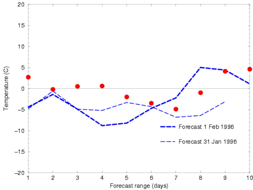
Figure 36 : The same as figure 1, but with verifying 12 UTC observations. Both forecasts are systematically too cold and when they verify on day 6, it is probably due to an additional error, a wrongly forecast synoptic pattern, which happens to compensate the systematic error.
