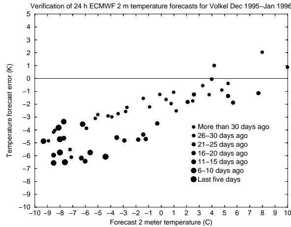
Figure 17 : A scatter diagram which depicts the relation between forecast 2 m temperature values and the forecast error. By varying the size of the circles the actuality of the values can be assessed. The mean error of about -4^{\circ}\text{K} does not correspond to any “flat bias”, but rather a systematic, almost linear relationship ( \text{error} = -2.0 + 0.4 \times \text{forecast} ) which can be explored to correct the forecasts.
