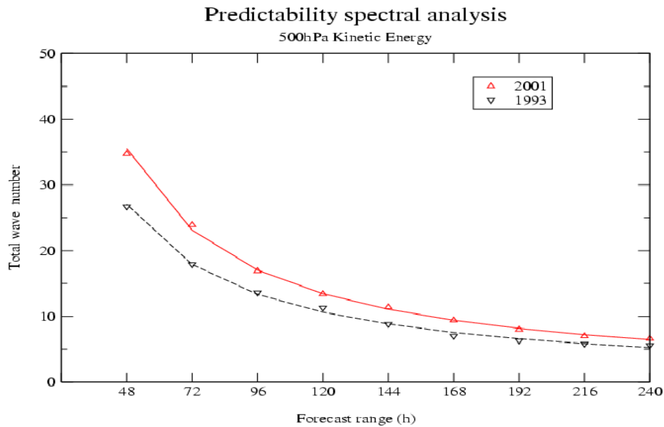
Figure 24 : The relation between the scale of an atmospheric feature at 500 hPa, measured by the number of spectral components needed to describe it, and its predictability. Forecasts beyond six days normally contain useful information only in the first 10-15 spectral components. Since 1993 the predictability measured in this way has increased by two days.
