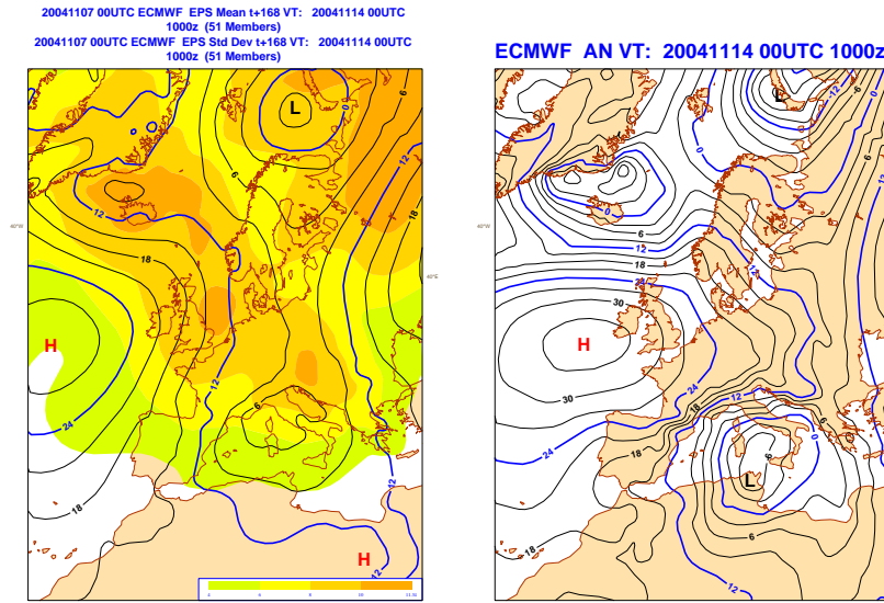
Figure 31 : D+7 ensemble mean (solid contours) and spread (shaded) of 1000 hPa Z compared with the verifying analysis (right). The high pressure over the Atlantic, northerly flow over Europe and the cyclogenesis over the Mediterranean sea were already in place 7 days before. The high value of the spread highlights regions where uncertainty is higher. However the spread is also very sensitive to displacement of gradients. It tends to be higher in areas with larger gradients.
