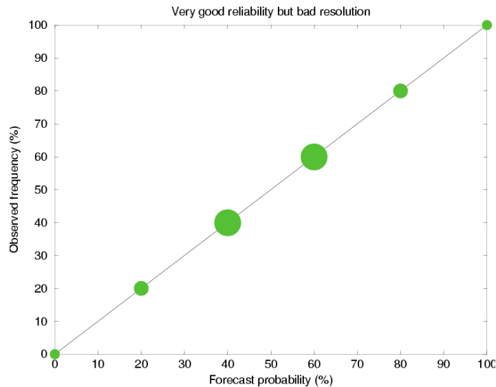
Figure 20 : An example of verification of a probabilistic forecast system with good reliability, but poor resolution. Most forecasts are centred around the climatological mean, with few cases when it provides confident forecasts (low or high probabilities).
