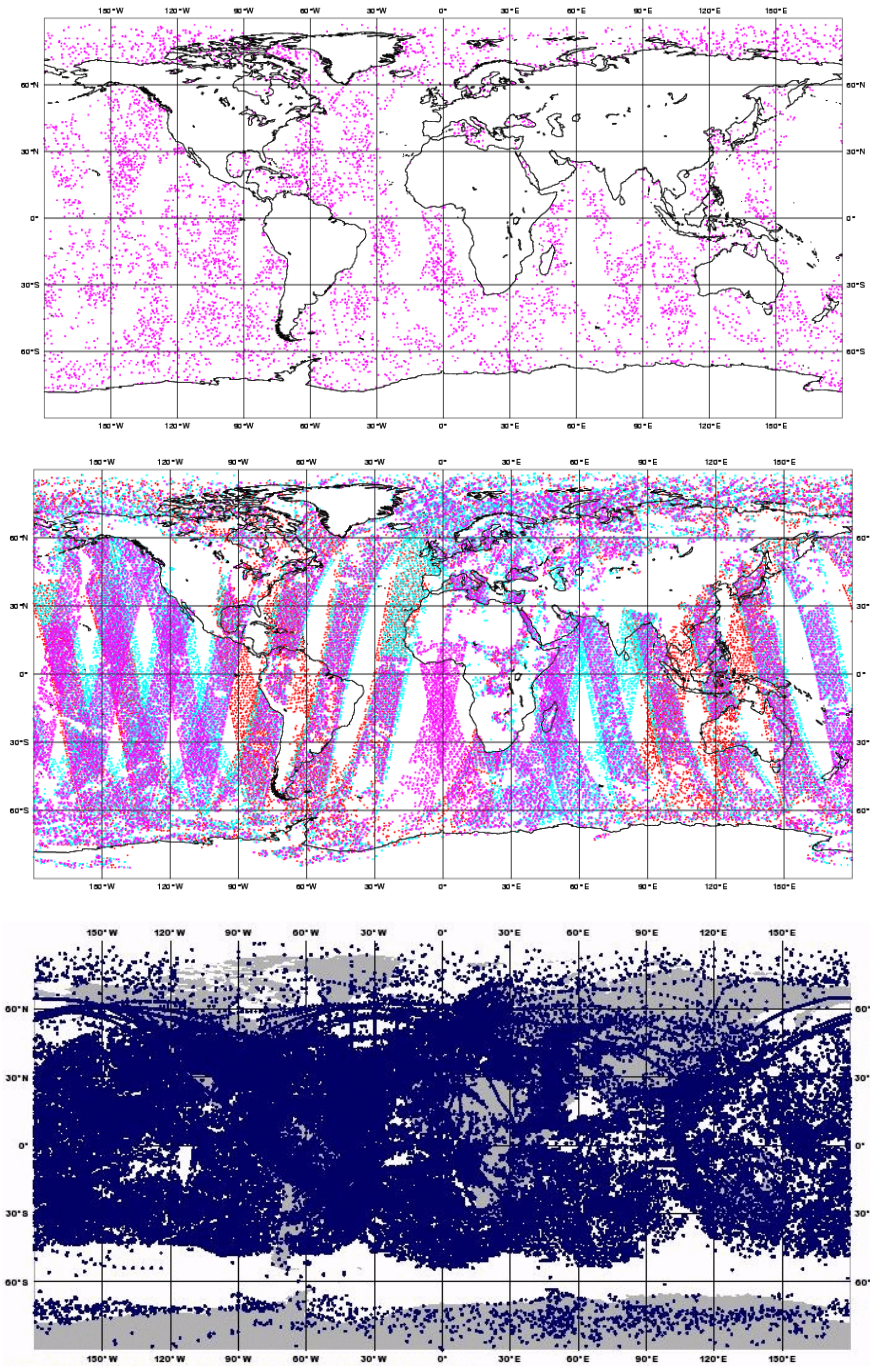
Figure 7 : Example of data coverage of used data during a day. From the top : a) infrared lower tropospheric channel from AQUA satellite, b) microwave lower tropospheric channel from three satellites (AMSU-A ch. 5 from NOAA-15, NOAA-16m AQUA), c) composite of conventional observations (surface + radiosoundings + aircrafts) and atmospheric winds derived by satellites. As it is apparent, despite a good global coverage there are land areas (Sahara, Siberia, Arctic and Antarctic) where the data coverage in the low troposphere is still sparse.
