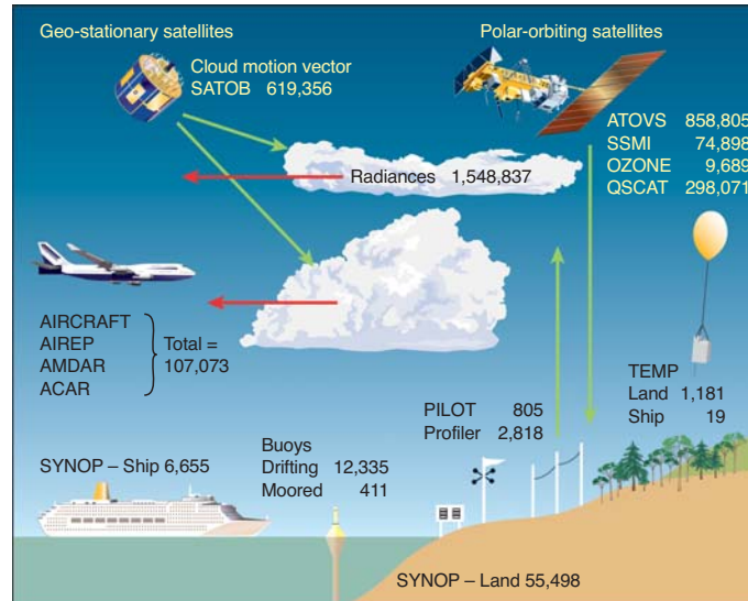
Figure 8 : 24h summary of observations received at ECMWF, 5 July 2004
