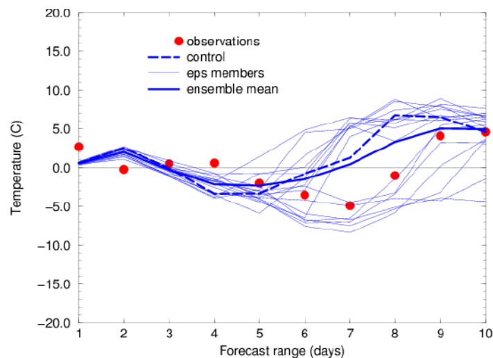
Figure 42 : The same as figure x2, but after statistically derived corrections have been applied to all the EPS members. Now the whole EPS plume was very realistic and that the substantial minority which indicated a prolonged cold period verified. Note that the statistical correction has reduced the spread of the plume to less than 15 K.
