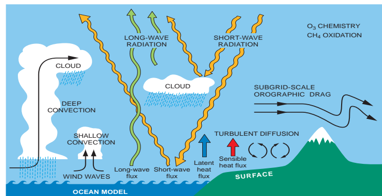
Figure 4 : Main physical processes represented in the ECMWF model.
