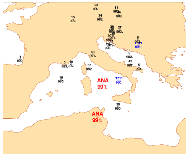
Figure 33 : Positions and minimum pressure of the lows below 995 hPa predicted by the EPS and T511 7 day before the event (20041114 00UTC, the same as Fig.24). EPS members are marked in black, T511 in blue and the verifying analysis in red. The EPS gave indications for a surface low development in the area but the position of the low was in general misplaced to the north. Note the mismatch has been smoothed out by the ensemble mean, compare with figure 24.
