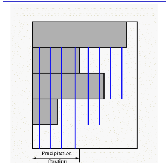
Figure 5 : Precipitation is treated separately in clouds and clear skies. The figure shows how model clouds cover areas which vary with height. Only a fraction of the grid box is covered by precipitation at all levels, including the surface.
