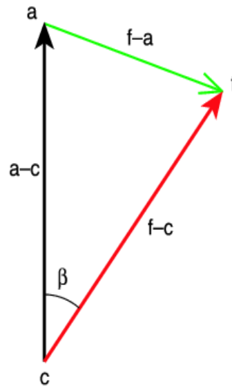
Figure 48 : The same analysis can be conducted in graphical form in a phase-space, using vector algebra where the observed anomaly a-c and the forecast anomaly f-c are represented by vectors of length A_f and A_a separated by an angle \beta . It can be shown that the ACC = \cos(\beta) and that the distance a-f is proportional to RMSE.
