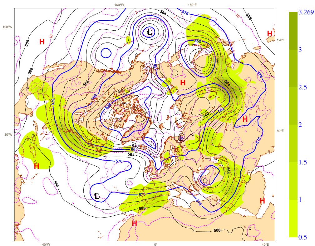
Figure 13 : The RMS of initial perturbations of temperature at 700 hPa 04 May 2005 00 UTC (shaded) plus 500 hPa Z (black contour) and T at 700 hPa (pink contour) as a reference field. The system has identified strong baroclinic regions over Asia and the east coast of USA as particularly sensitive to possible uncertainties in the analysis. Note also the Caribbean region has been identified (Tropical SV).
