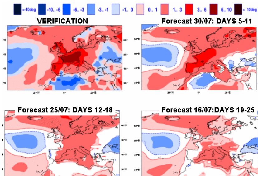
Figure 46 : The extreme heat wave that affected large parts of western and southern Europe in August 2002 was well indicated by the monthly forecast system. The figure shows the ensemble mean of the anomalies (relative to the model climate) for three monthly forecasts initialized on 16, 25 and 30 July valid 3-9 August.
