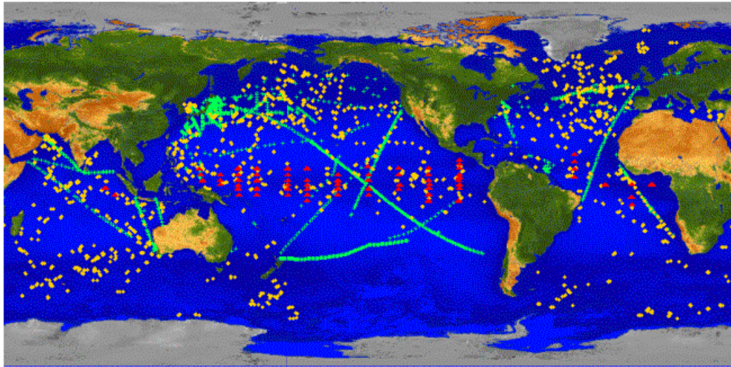
Figure 45 : The data coverage for May 2003. Red dots are moored buoys, yellow are ARGO floats, green XBT (expandable bathy thermographs). During the last years there has been a dramatic increase of real-time oceanographic observations.
