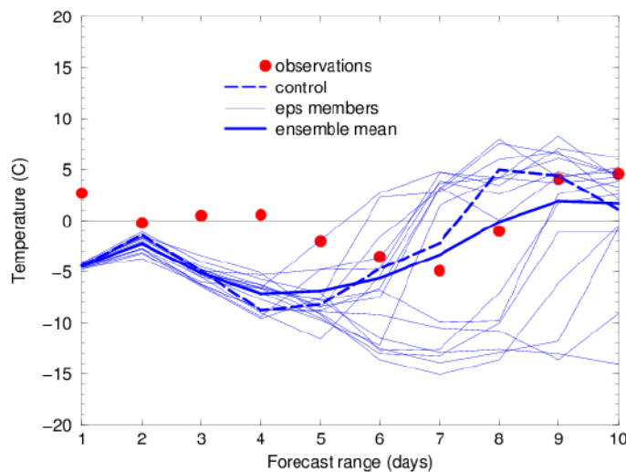
Figure 41 : The same as figure x, but now with the output from the EPS. The non-perturbed Control forecast from 1 February is supported by more than half of the members, indicating a return to milder conditions after about five days. A substantial minority support the forecast from the previous day, 31 January, that it will stay cold during most of the ten-day period. However, the verifying observations show that the whole forecast is rather poor. The spread during the last days was almost 25°K.
