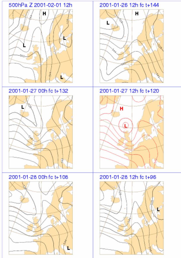
Figure 25 : An example of forecast “jumpiness” from the end of January 2001. Over a period of two days, the D+4 to D+6 are quite consistent, only with the exception of the D+5 from 27 January.
