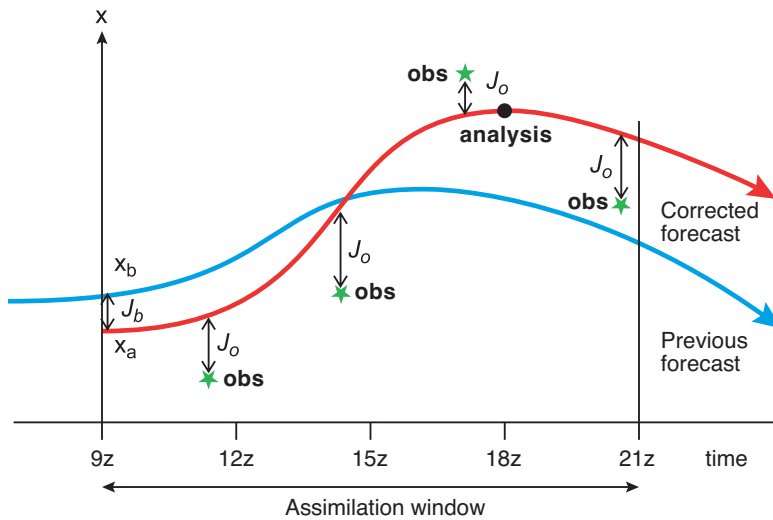
Figure 9 : A schematic illustration of the 4Dvar analysis
