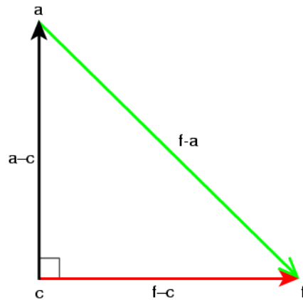
Figure 49 : For the case when \beta=90^\circ the forecast and analysis are uncorrelated and ACC=\cos\beta=0
