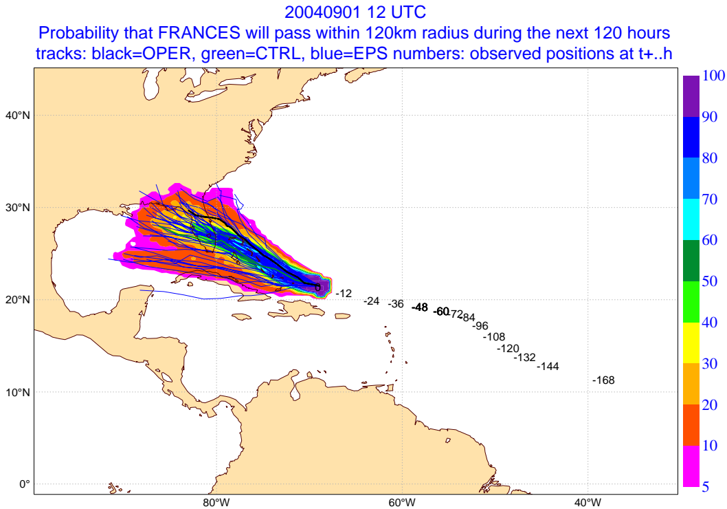
Figure 35 : Strike-probability map for hurricane Frances, valid for a five days period starting at 12UTC 01 September 2004. Strike probabilities are shaded, high-resolution and EPS Control unperturbed tracks are in black and green respectively. Blue lines are the perturbed EPS members. Black numbers refers to the position of the cyclone -n hours before.
