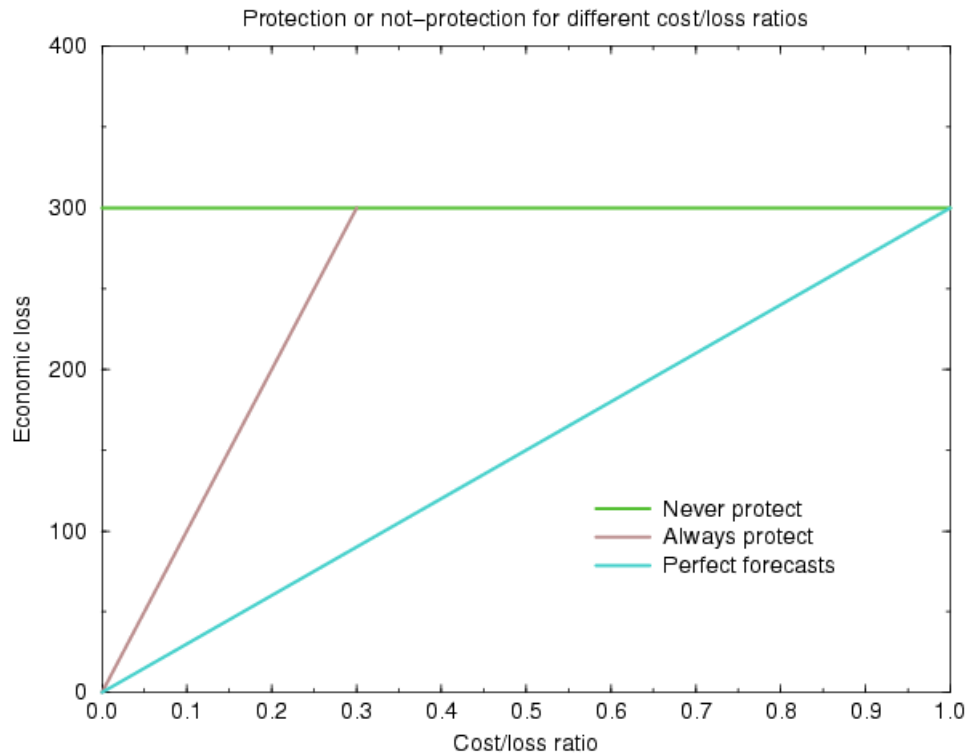
Figure 22 : The figure above illustrates schematically the situation in a certain location where there is a climatological risk of 30% having bad weather (rain) on a particular day
