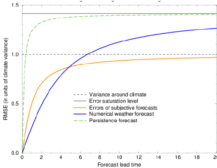
Figure 28 : Same as figure but with the error growth of a NWP forecast model schematically indicated. At some stage the NWP is less accurate than climatological information and before that worse than a pre-NWP forecaster.
