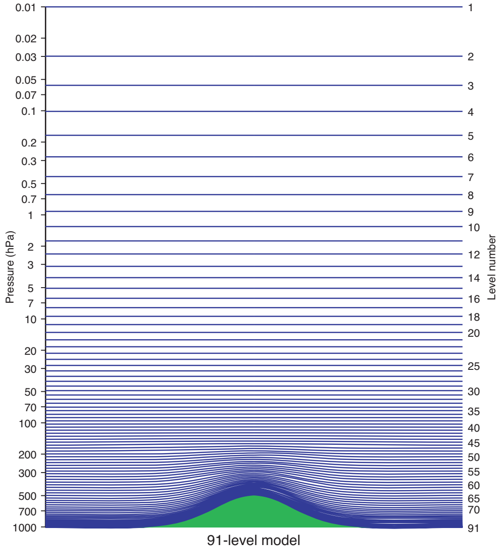
Figure 2 : Distribution of vertical levels in the T799 model.
