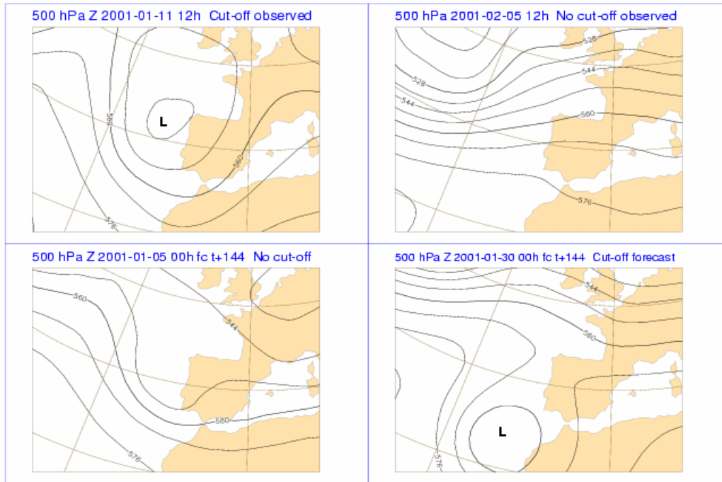
Figure 30 : The maps to the left show a case when the forecast failed to forecast an existing cut-off, the maps to the right a case when a cut-off was forecast which never occurred. Verifications over a long periods show that approximately the same number of cut-off are forecast as are observed - they just do not always match at a D+6 range.
