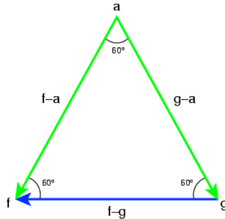
Figure 51 : Figure 50 “watched” from the upper right displays the three vectors (f-a), (g-a) and (f-g) and their mutual correlations, which is the cosine of their intermediate angles 60°, which yields correlations of 0.5.
