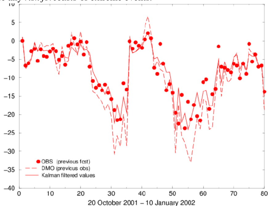
Figure 40 : In the case the forecast variance is larger than the observed the statistical interpretation can equally well correct for this.
