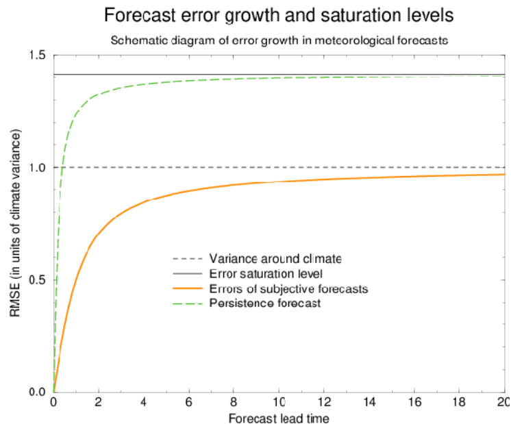
Figure 27 : A schematic representation of the pre-NWP accuracy of weather forecasts measured in RMSE with the climatological variance (the accuracy of a climatological statement) as a norm. The time unit at the x-axis is arbitrary. While the subjective forecaster was careful to make less and less detailed forecasts, the persistence forecasts became less accurate than climate in quite early forecast ranges converging to a 41% higher error level.
