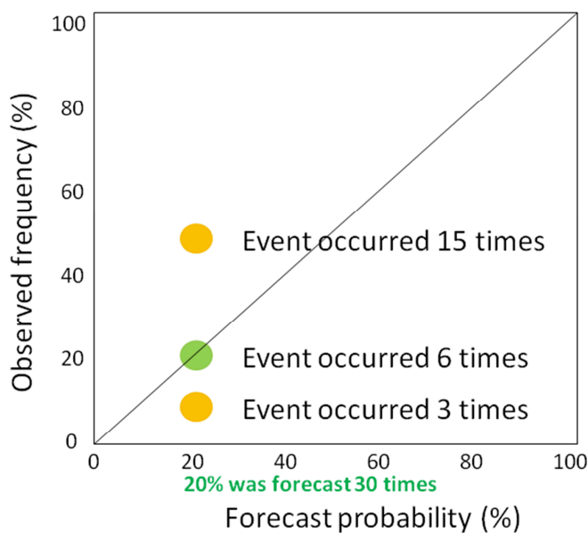
Figure 81: Schematic explanation of the reliability diagram. Out of thirty 20% probability forecasts, the predicted event should verify six times, i.e. in 20% of the time, not more, not less.
