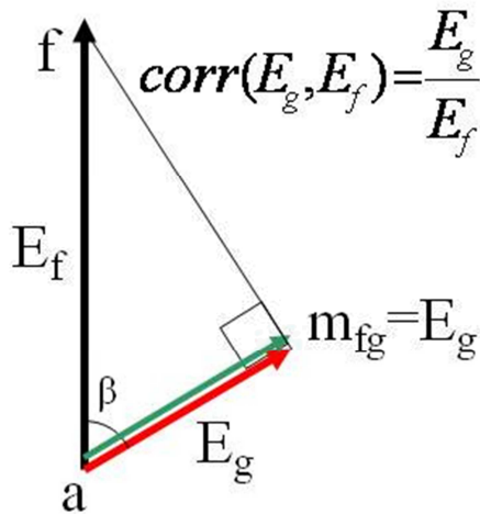
Figure 75: For certain relations between forecast accuracy and forecast error correlation no combination will be able to reduce the RMSE.
