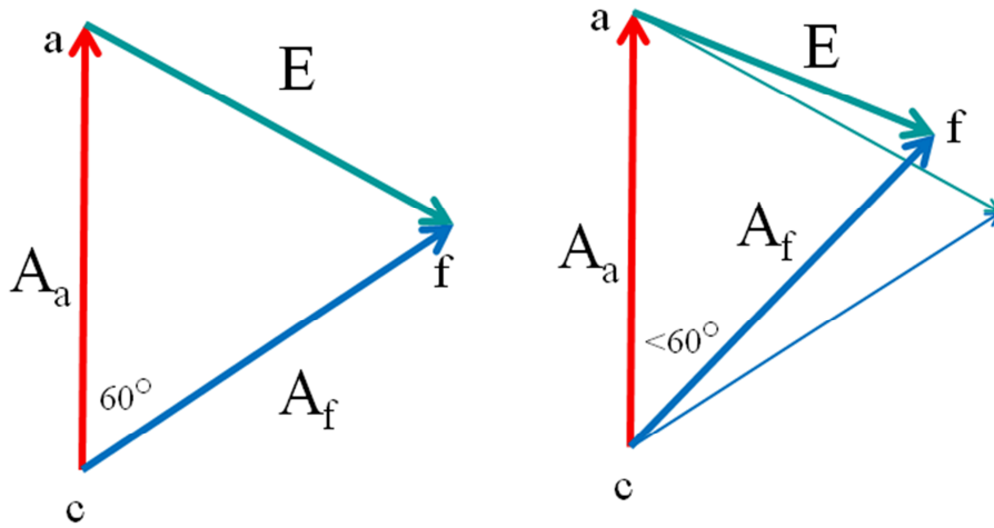
Figure 70: When the ACC=50%, i.e. the angle between the anomalies (a-c) and (f-c) =60°, the RMSE= A_a , the atmospheric variability (left). When ACC>50% the RMSE is smaller. An ACC=60% is agreed to indicate the limit of useful synoptic forecast skill.
