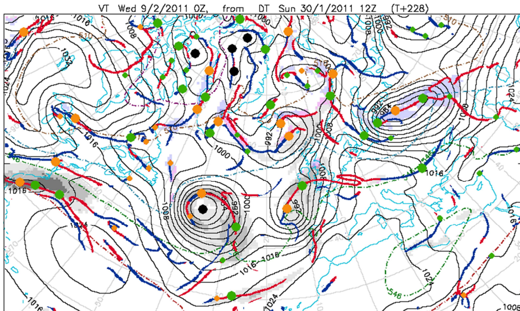
Figure 58: A still image of EPS member 15 on 30 January 2011, 12 UTC + 228 hour forecast. Likely positions of fronts and troughs are indicated by lines and important synoptic features by filled circles.
