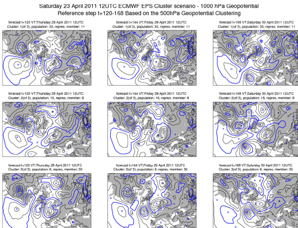
Figure 59: The most representative 1000 hPa members selected to describe the clustering of the forecast 23 April 2011, 12 UTC +120 to +168 hours.
