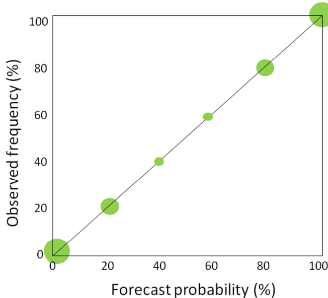
Figure 82: Probabilities with good sharpness. The probabilities cluster as far away as possible from the climatological frequency, here assumed to be 50%.
