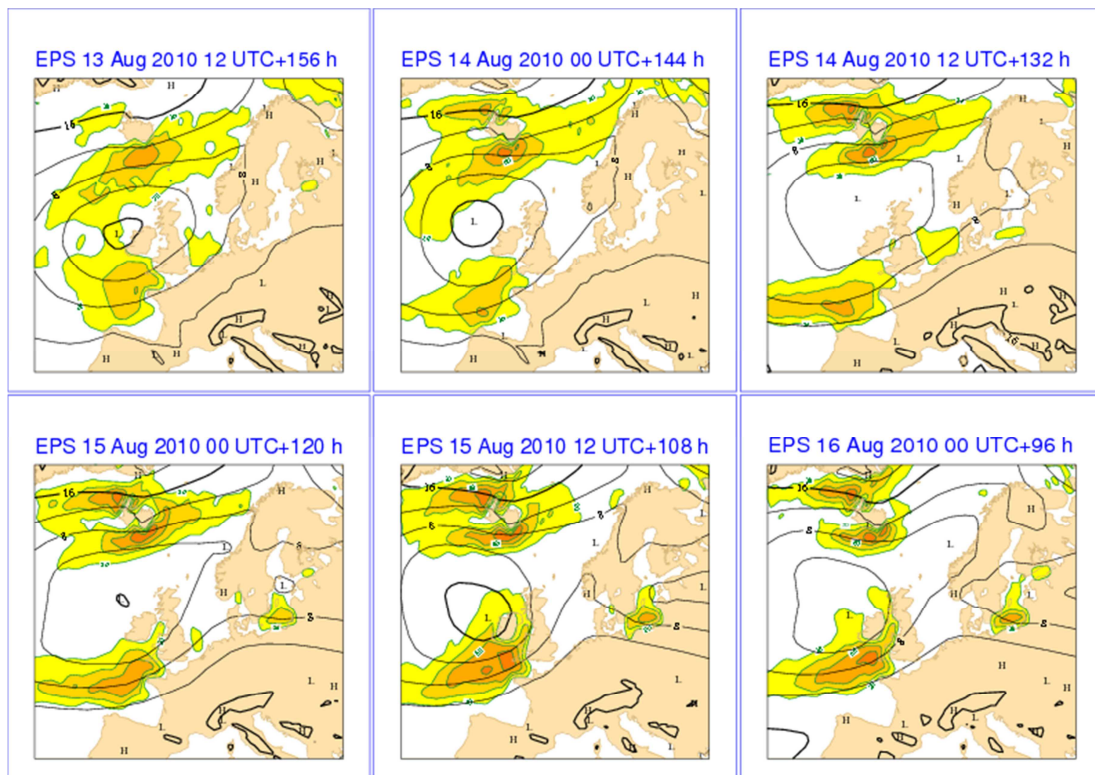
Figure 32: 1000 hPa EPS from 13 August 12 UTC +156 h to 16 August 00 UTC +96 h, all valid at 20 August 00 UTC. Full lines are the 1000 hPa geopotential EM overlaid by the probabilities of wind speeds > 10 m/s. Probabilities are coloured in 20% intervals starting from 20%. Compare with Figure 18 and Figure 19.
