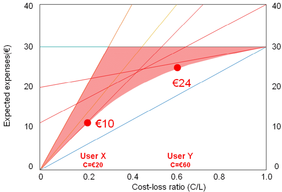
Figure 80: The same figures but with the expected expenses indicated for cases where different end-users take action after receiving probability forecasts. The general performance (thick blue line) is now closer to the performance for perfect forecasts.
