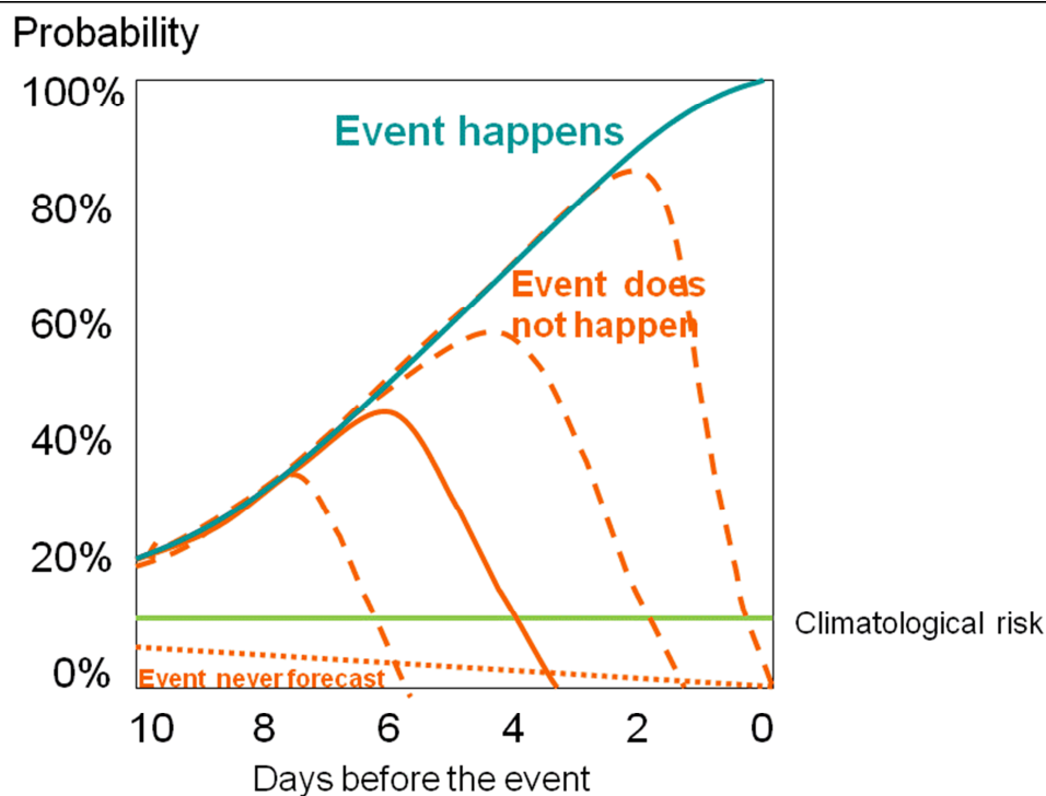
Figure 34: A schematic illustration of an average probability development for a specific location over ten days. The climatological probability of some anomalous event (lime green line) is where all probability forecasts start. If very few or no EPS members forecast the event and there are no other indications, the probability gradually reduces to zero, as the verifying time approaches (orange dotted line). On the other hand, if ensemble members forecast the event with increasing frequency, the probabilities increase (turquoise line). However, at any lead time, the increase may stop and fall back to the lower levels or to zero (dashed orange line). In this particular scenario, at day 6 there is a 50% chance that the event will verify and, consequently, a 50% probability that the event will not occur and that the probabilities will later decrease to zero (continuous orange line).
