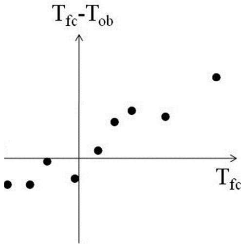
Figure 63: A scatter diagram of forecasts versus forecast error. Warm forecasts appear too warm, cold forecasts appear too cold. If the forecasts are short range, it is reasonable to infer that the system is over-active, overdeveloping warm and cold anomalies. If, on the other hand, the forecasts are well into the medium range, this might not be the case. Due to decreased forecast skill, predicted anomalies tend to verify against less anomalous observed states.
