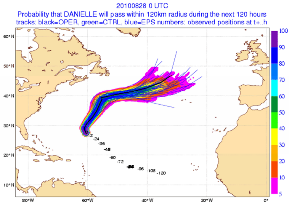
Figure 55: Strike probability map for tropical storm Danielle from the 28 August 2010, 00 UTC.
