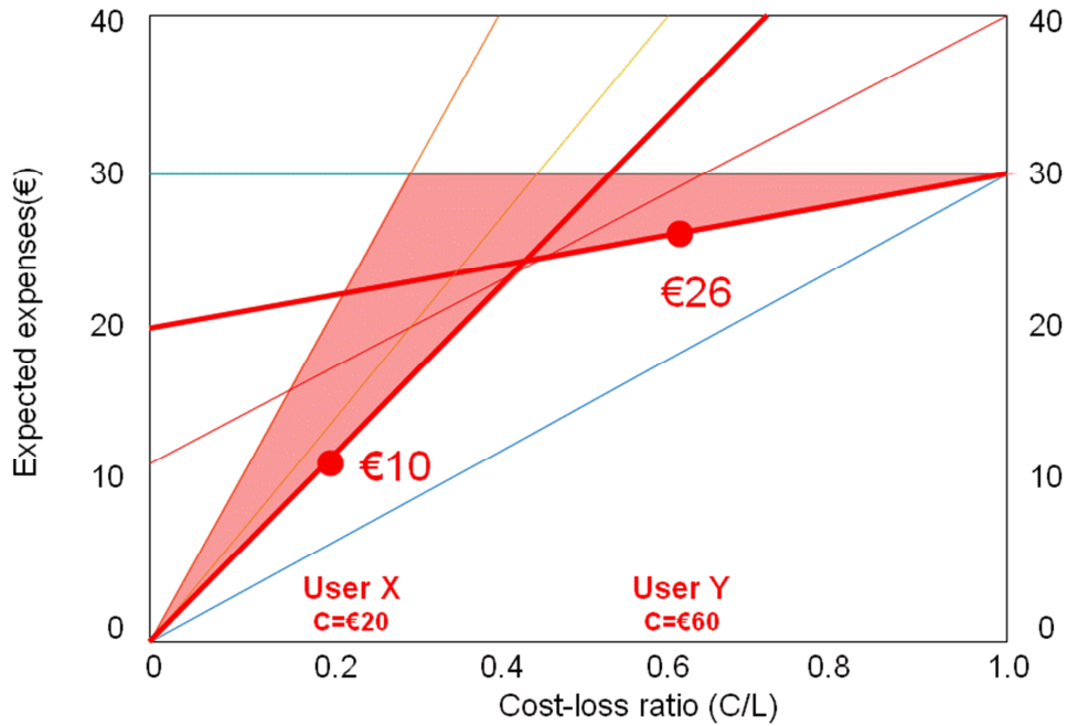
Figure 79: The expected daily expenses when the end-users are free to interpret the “don’t know” forecast either as “rain”, if they have a low c/L ratio, or as “no rain”, if their c/L ratio is high.
