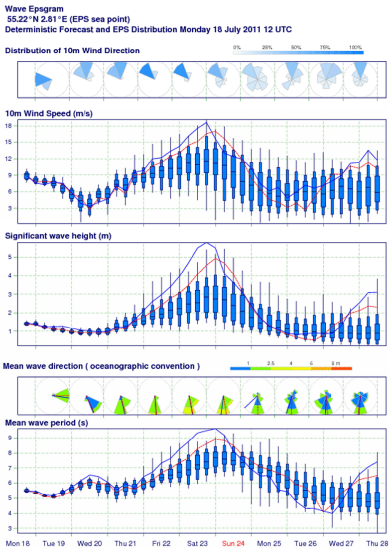
Figure 49: An example of a wave EPSgram for the North Sea 18 July 2011, 12 UTC. A north-westerly wind is forecast to increase over the location, giving rise to amplified waves with increasing periods. The mean wave direction indicates that during the weekend the waves travel mainly to the south with a higher proportion of large waves.
