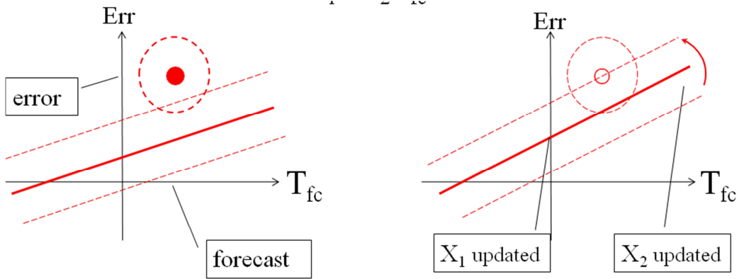
Figure 96: A schematic illustration of the workings of an adaptable MOS by Kalman filtering. At a given time the error equation has a certain orientation (full red line) with a certain estimated uncertainty (red dashed lines). A forecast is verified and yields an error (red filled circle) that does not normally fall on the error line. Depending on the interplay between the equation uncertainty and the verification uncertainty (dashed red circle), the error equation line is translated and rotated to take the new information into account, after which this information is discarded.
