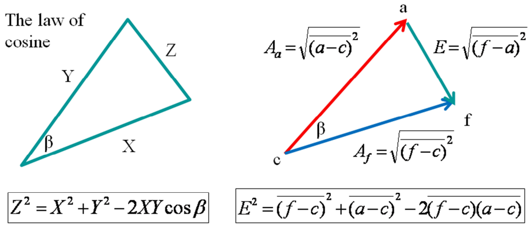
Figure 68: The relationship between the cosine theorem and the decomposition of the RMSE.
