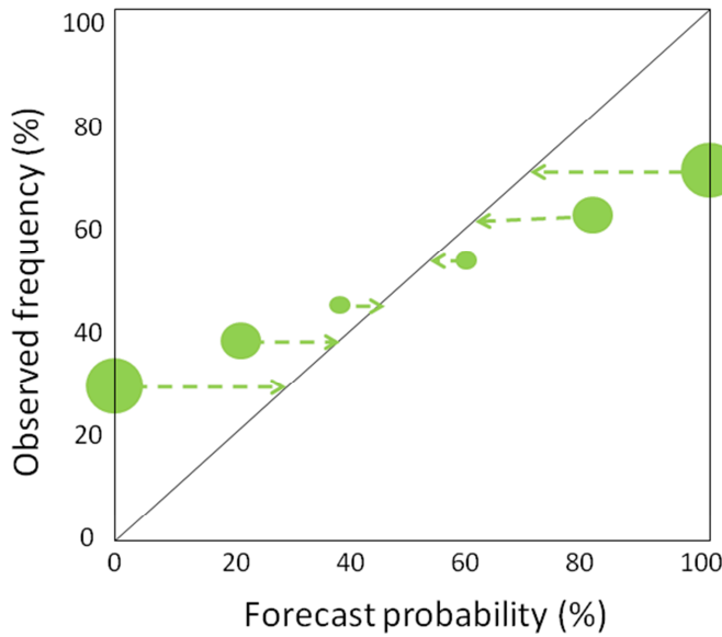
Figure 92: The probability distribution from an overconfident forecast system is calibrated, limiting the range from 0% - 100% to 30% - 70%.
