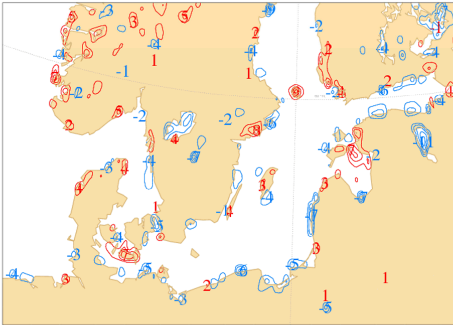
Figure 12: The difference in 2 m temperature between the operational model and the EPS Control for 23 April 2011 00 UTC + 12h. The maximum and minimum differences are indicated as integers. The interval is 2°C. The differences are largest where the discrepancy between the operational and EPS Control land-sea mask or orography is largest.
