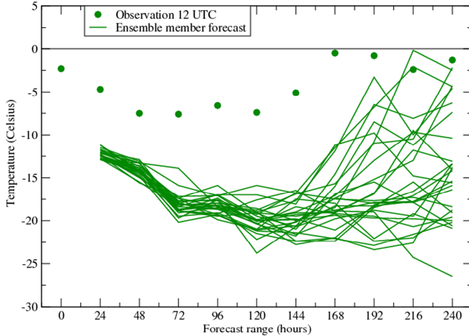
Figure 97: A plume diagram for Tromsø, 12 February 2011. The forecast is too cold with 50-100% probabilities of temperatures < -15°C.
