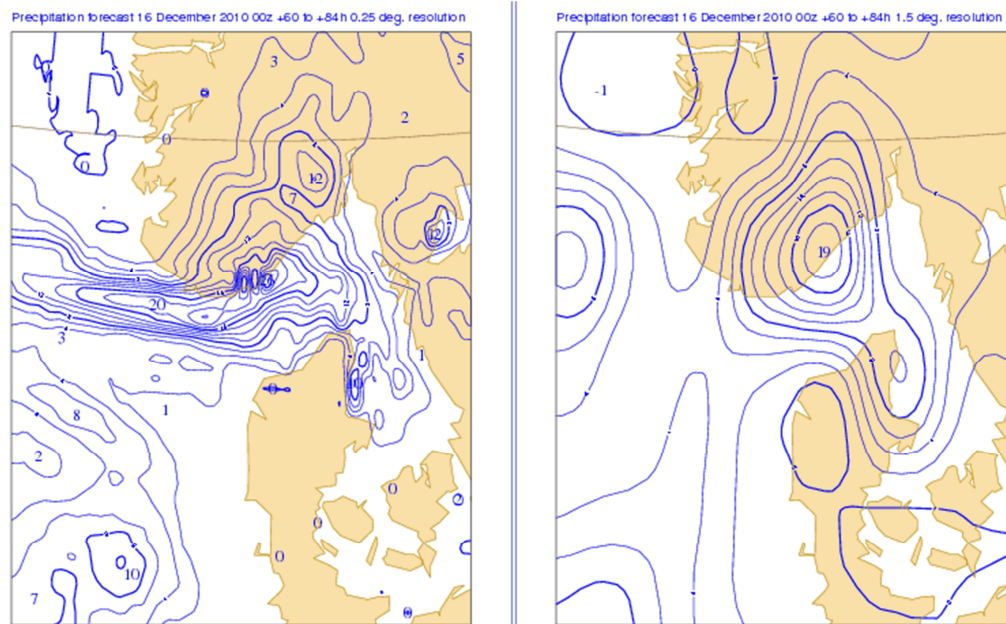
Figure 9: Example of the effect of inappropriate interpolation of precipitation fields. To the left the forecast is interpolated in a 0.25 \times 0.25^\circ grid, to the right in a 1.5 \times 1.5^\circ grid.
