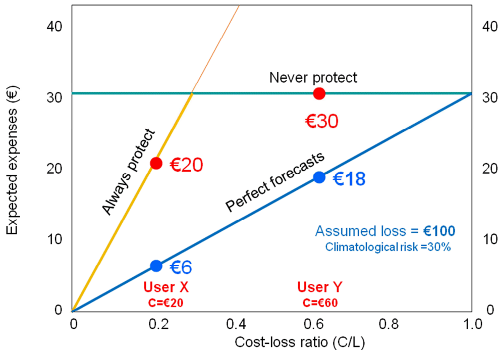
Figure 76: The triangle defined by the expected daily expenses for different costs ( c ), when the loss ( L ) is 100€. End-users who always protect increase their expenses (yellow), end-users who never protect lose on average 30 € per day. Even if perfect forecasts were supplied, protection costs could not be avoided (blue line). The triangle defines the area within which weather forecasts can reduce the expected expenses.
