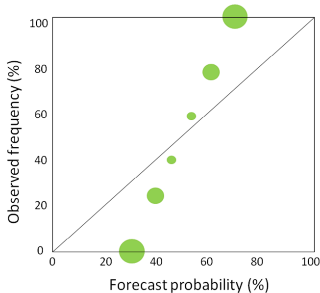
Figure 85: Probabilities indicating reluctance to use very high or low probabilities. The probability forecasts are under-confident.
