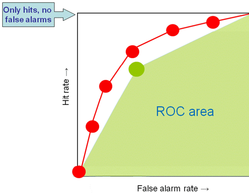
Figure 91: The area underneath the points, joined by straight lines, defines the ROC area, which is, ideally, 1.0 and at worst 0.0. Random forecasts yield 0.5, the triangular area underneath the 45° line.
