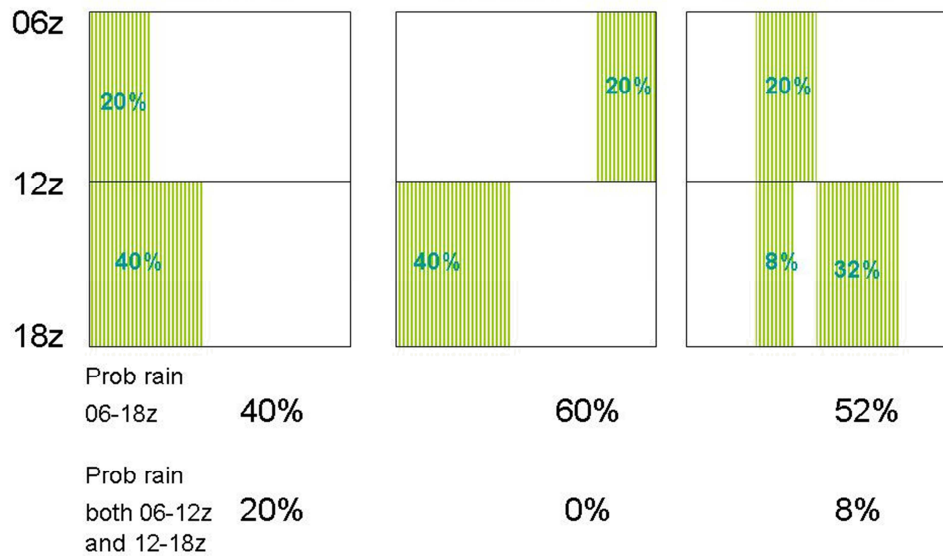
Figure 35: If the events in the two adjacent time intervals are non-correlated, the combined probability is (1 - (1 - 0.4)(1 - 0.2)) = 52\% (far right figure). If they are correlated, so that rain in the first interval is followed by rain in the second, the probability for rain at any time during the whole period is 40% (far left figure). If they are anti-correlated, so that rain in the first period is followed by dry conditions in the second, and dry in the first period is followed by rain in the second, then the total probability is 60% (centre figure).
