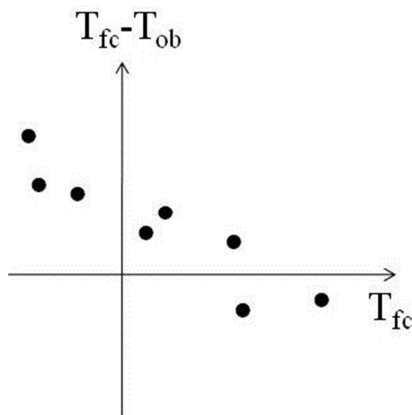
Figure 60: A convenient way to differentiate between "unconditional" and "conditional" biases is to plot scatter diagrams, with forecasts vs. forecast errors or observations (analyses) vs. forecast error. From the slope and direction of the scatter in these diagrams it is also possible to find out if the forecasts are over- or under-variable. In this case the colder the forecasts the larger the positive error, the warmer the forecast the larger the negative error. This implies that cold anomalies are not cold enough and warm anomalies not warm enough, i.e. the forecasts are under-variable.
