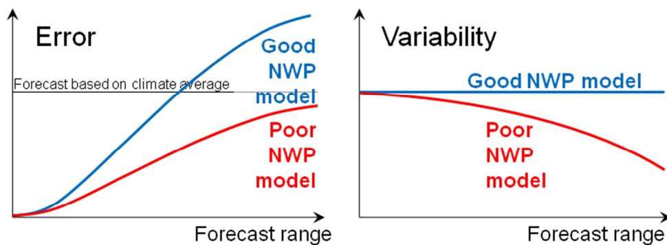
Figure 30: The root-mean-square error and variability of two NWP systems: one a good state-of-the-art high-resolution NWP model (blue curve in left figure), the other a poor NWP model due to excessive diffusion or coarse numerical resolution (red curve in left figure). The errors of the good model approach a high error level because it is able to represent the whole spectrum of resolvable atmospheric scales throughout the forecast (straight blue line in the right figure), while the errors of the bad model approach a lower level because it suffers from a gradual reduction of the scales and thereby the variability (red curve in the right figure).
