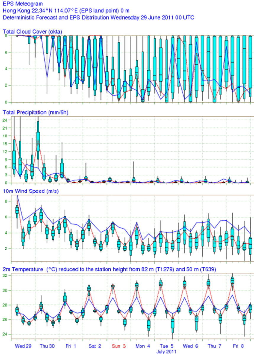
Figure 48: The 10-day EPSgram for Hong Kong, based on the ECMWF forecast from 29 June 2011, 00 UTC. The discrepancy between the deterministic forecast (blue line) and the EPS Control (red dotted line) is due to the grid-point definitions. Thanks to its higher resolution, the deterministic model's closest grid point is fairly close to Hong Kong, whereas the closest grid point in the EPS Control (and all the members) is situated on mainland China, with its warmer and less windy climate.
