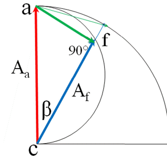
Figure 72: Damping the forecast variability A_f will minimize the RMSE, if it becomes orthogonal to the forecast. This happens when A_f = ACC \cdot A_a and the forecast vector f-c varies along a semi-circle with a radius equal to half A_a .
