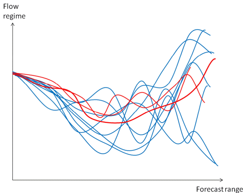
Figure 37: The same as Figure 36 for the case when the deterministic forecasts are consistent, with smaller spread than the ensemble.
