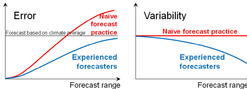
Figure 31: The same as figure 30 but for two different forecast practices: one experienced practice which disregards or damps less likely synoptic features, the other which naïvely reads off the raw output from a state-of-the-art NWP model. The errors of the experienced practice (blue curve in the left figure) approach a low error level because of a gradual reduction of the less predictable scales and thereby the forecast variability (blue curve in the right figure), while the errors of the naïve practice approach a higher error level (red curve in the left figure) because the forecasts maintain the whole spectrum of resolvable atmospheric scales for all lead times irrespective of whether they are predictable or not (straight red line in the right figure).
