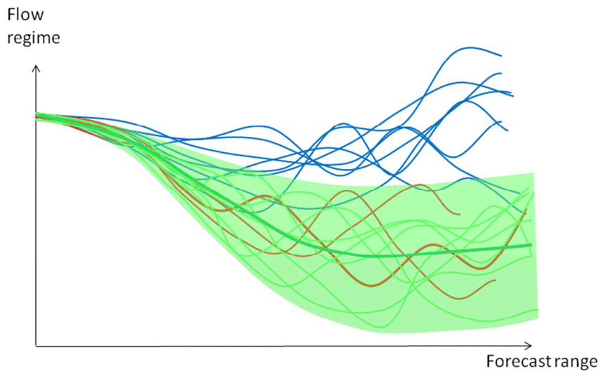
Figure 43: A schematic illustration to show how the latest operational forecasts (red lines) are combined with the previous EPS (green lines, the thick line being the EM).
