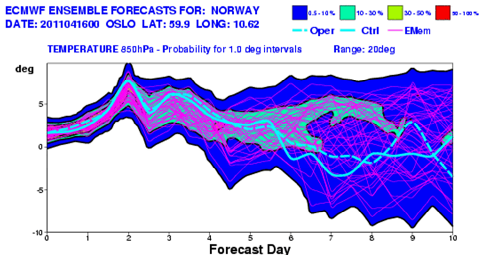
Figure 28: A plume diagram for Oslo 16 April 00 UTC. The ensemble forecast indicates a bi-modal development between days 5 and 7, whereas the operational forecast and the Control follow one branch.
