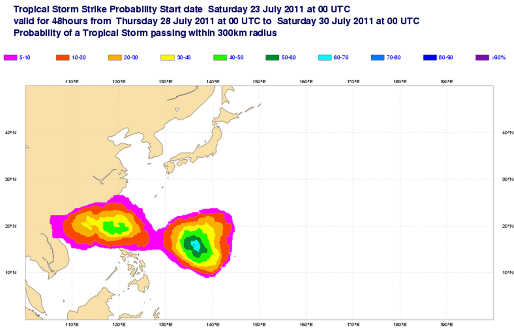
Figure 57: The Tropical Storm Strike Probability chart from Saturday 23 July 2011, indicating the probability of the passage of two not yet developed storms, within a 300 km radius, between 5 and 7 days ahead, i.e. during the 48 hours between Thursday and Saturday 28-30 July 00 UTC. The western system developed into tropical storm NOCK-TEN and briefly reached typhoon status with maximum sustained winds of 75 mph late on Tuesday evening. The eastern system developed into a tropical depression on the 25 th , a tropical storm, named MUIFA, on the 28 th and a typhoon on the 30 July.
