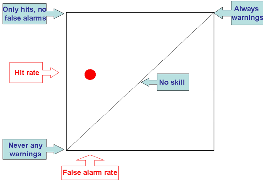
Figure 89: The principle of the ROC diagram: a large number of probability forecasts are turned into categorical forecasts depending on whether the probability values of individual forecasts are above or below a certain threshold. The false alarm rate and the hit rate are calculated, thus determining the position in the diagram (red filled circle).
