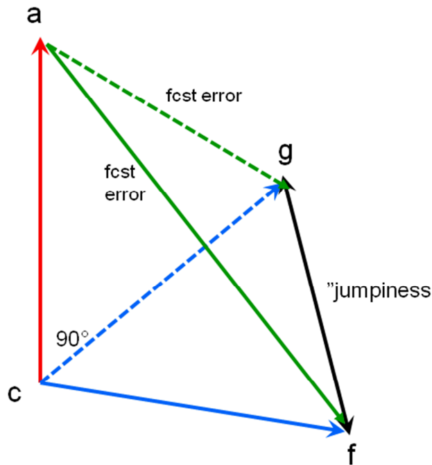
Figure 73: A 3-dimensional vector figure to clarify the relation between forecast jumpiness and error. Two forecasts, f and g , are shown at a range when there is no correlation between the forecast and observed anomalies ( f-c ), ( g-c ) and ( a-c ). The angles between the three vectors are 90^\circ . The angles in the triangle a-f-g measure up to 60^\circ which means that there is a 50% correlation between the “jumpiness” ( g-f ) and the errors ( f-a ) and ( g-a ). The same is true for the correlation between ( f-a ) and ( g-a ).
