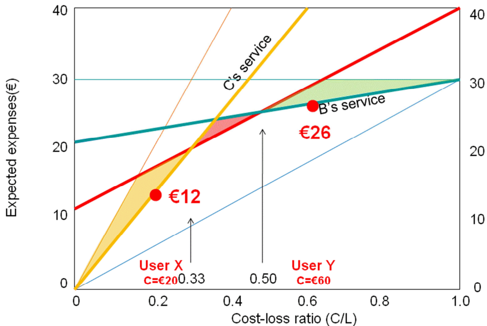
Figure 78: The cost-loss diagram with the expected expenses according to forecasts from agencies B and C for different end-users, defined by their cost-loss ratios. Weather service A is able to provide only a section of the potential end-users, the ones with C/L-ratios between 33 and 50%, with more useful forecasts than B and C. The green and yellow areas indicate where X and Y benefit from the forecasts from agencies B and C respectively.
