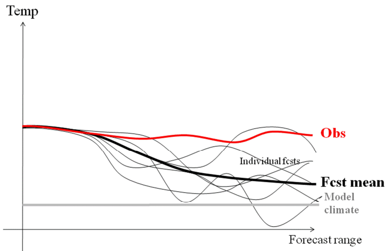
Figure 64: A sequence of consecutive NWP forecasts (thin black lines, their mean (thick black line) and the observations (red line). Forecasts starting in an anomalous state are less likely to forecast even more extreme conditions. With increasing lead time and decreasing skill the forecasts will tend to cluster increasingly around the climate average and give an impression of increasing ME. The mean error will therefore give the false impression of a drift in the model climate.
