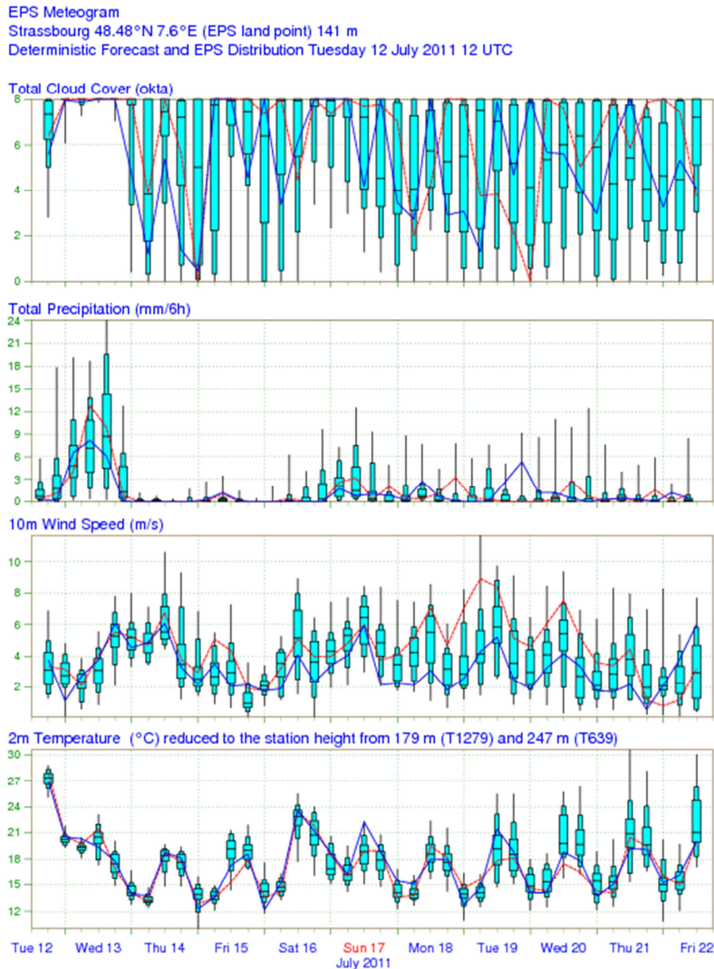
Figure 46: The 10-day EPSgram for Strassbourg, based on the ECMWF forecast from 12 July 2011, 12 UTC. The expected 6-hourly rain on Wednesday 13 and Sunday 17 July cannot easily be converted into 24-hourly values. Blue lines indicate the operational deterministic high-resolution forecast, the dashed red lines the coarser resolution Control forecast.
