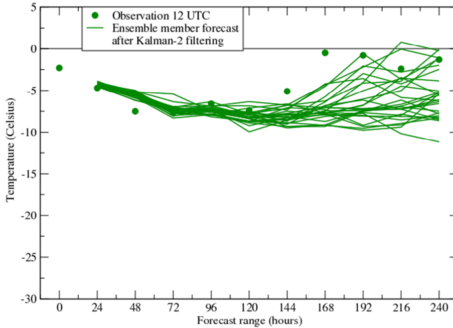
Figure 98: The same as Figure 97 but after the Kalman-filtered errors equation has been applied. Mild forecasts have hardly been modified, whereas cold ones have been substantially warmed, leading to less spread and more realistic probabilities with, for example, 0% probabilities for 2 m temperature <-15°C.
