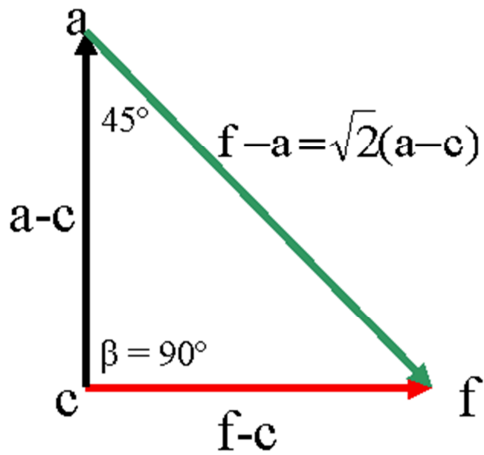
Figure 69: When the forecast and observed anomalies are orthogonal (i.e. uncorrelated) \beta=90^\circ and the forecasts (f-c) have on average errors equal to \sqrt{2} times A_a (the atmospheric variability) or the error of a climatological average.
