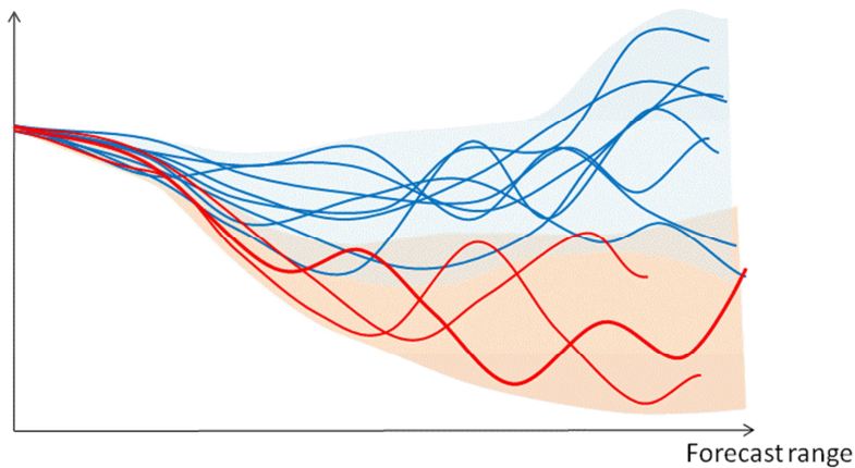
Figure 40: Same as Figure 36; an illustration of the combination of the EPS with the latest operational forecasts, as if they were two independent ensemble systems (blue and red shading).
