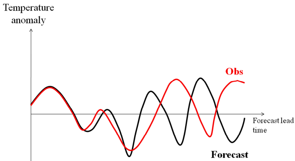
Figure 62: A schematic picture of a medium range forecast (black) and the verifying analysis. The forecast anomalies have about the same magnitudes as the verifying anomalies, but they are out of phase. This will yield a tendency for positive anomalies to verify against less positive or even negative anomalies, negative anomalies to verify against less negative or even positive anomalies.
