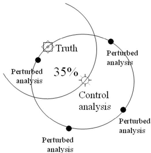
Figure 25: Although the perturbed analyses differ on average from the Control analysis as much as Control from the truth, for a specific gridpoint only 35% of the perturbed analyses are closer to the truth than the Control analysis.
