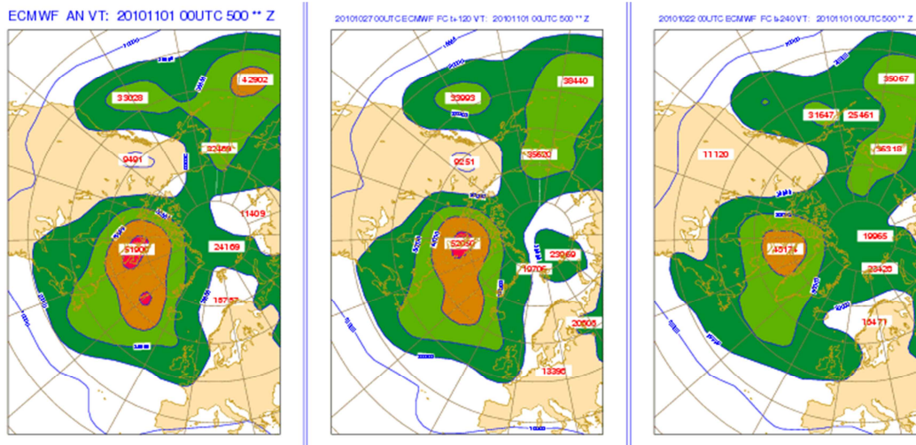
Figure 61: 500 hPa geopotential variability, October 2010 - March 2011. The standard deviation over the period is calculated for every grid point. The analysis (left) shows maximum variability between Greenland and Canada and in the North Pacific. This is well captured by the D+5 forecast (centre) and D+10 forecast (right) but with slightly decreasing values.
