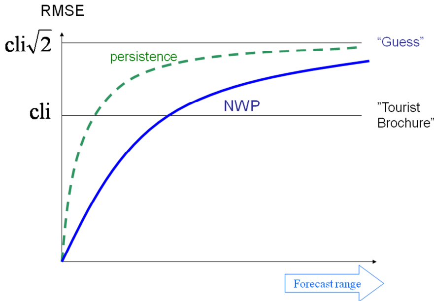
Figure 66: The error growth in a state-of-the-art NWP forecast system will at some stage display larger errors than a climatological average used as forecast and will, as do the errors of persistence forecasts and guesses, asymptotically approach an error level 41% above that of a forecast based on a climatological average
