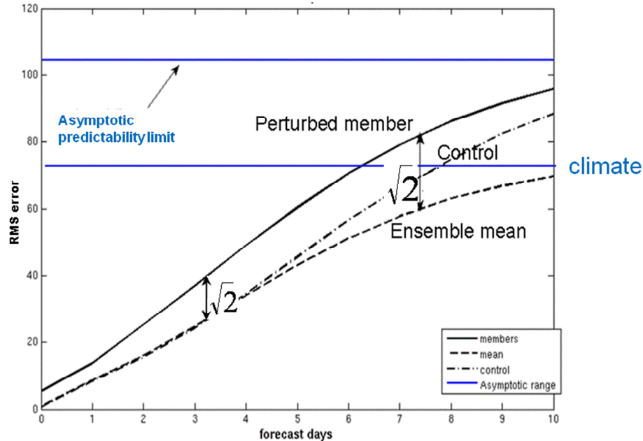
Figure 27: Schematic image of the RMS error of the ensemble members, ensemble mean and Control forecast as a function of lead-time. The asymptotic predictability limit is defined as the average difference between two randomly chosen atmospheric states. In a perfect ensemble system the RMS error of an average ensemble member is \sqrt{2} times the error of the ensemble mean.
