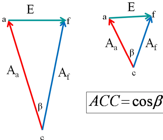
Figure 71: In situations with large variability around the climate average (left) relatively large RMSE can be associated with relatively large ACC (small \beta ) and (right) in situations with relatively small variability around the climate relatively small RMSE can be associated with small ACC (larger \beta ). For these cases the RMSE and ACC will give conflicting signals.
