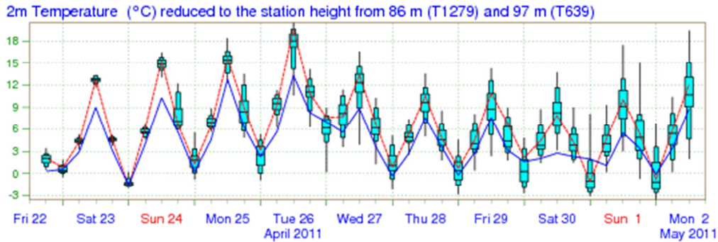
Figure 11: Part of an EPSgram for Kontiolahti in eastern Finland, 22 April 2011 12 UTC. The systematic difference between the operational model (blue line) and the EPS Control (red line) is around 5°C. Kontiolahti lies close to a small lake resolved in the operational model but not in the coarser EPS Control resolution (for more details about EPSgrams see Section 5.2).
