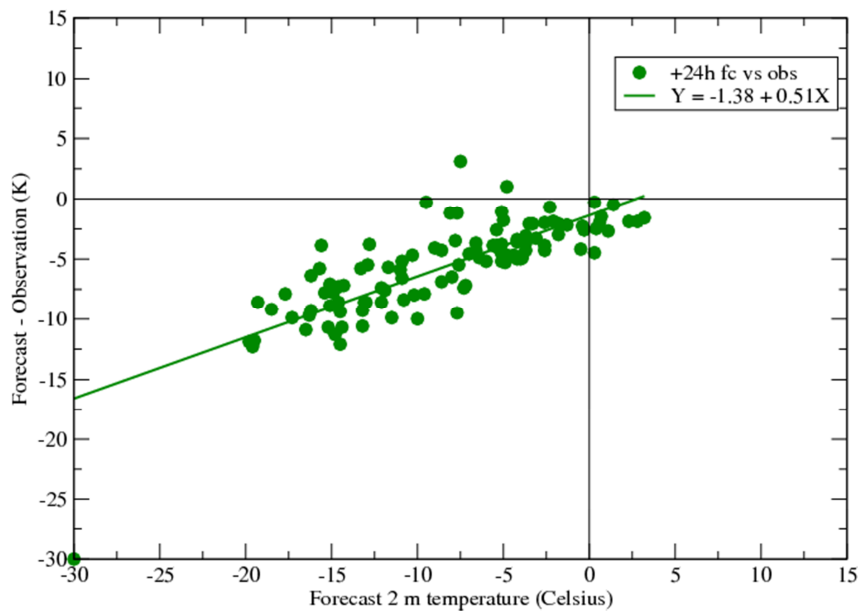
Figure 94: A scatter diagram of forecast errors versus forecast for Tromsø in northern Norway, November 2010 - February 2011. Cold temperatures are too cold and, as a whole, the forecasts overestimate the variability of the temperature.
