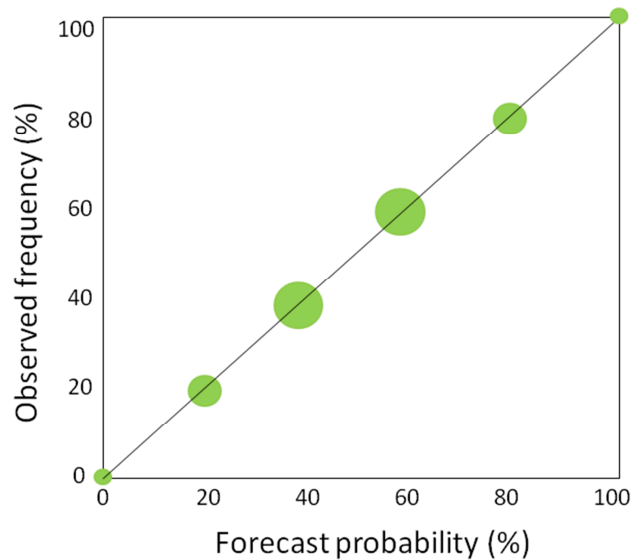
Figure 83: An example of a reliable forecast system with poor sharpness. When the predictability of a certain weather parameter is low, the forecasts might still be reliable but will tend to cluster around the climatological average.
