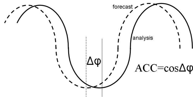
Figure 67: When the phase error \Delta\phi is larger than half a wave length, the scores will be worse than if there was no wave forecast at all.
