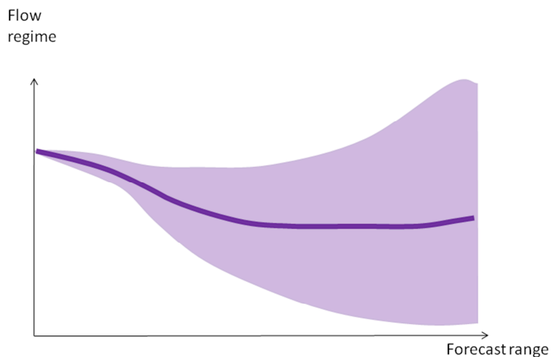
Figure 44: The resulting expanded ensemble, where the EM is the average of the two systems' EMs and the spread their combined spread.
