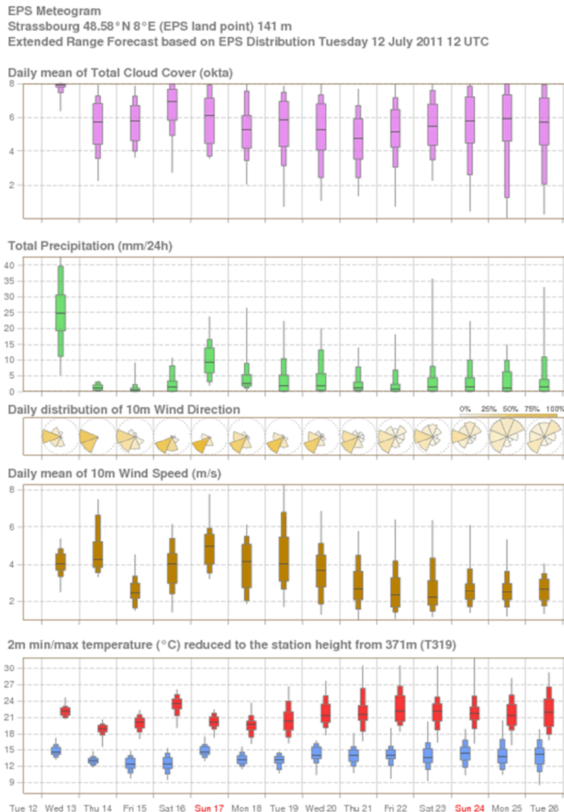
Figure 47: The 15-day EPSgram for Strassbourg, based on the ECMWF forecast from 12 July 2011, 12 UTC. Here, 24-hourly rainfall probabilities are computed, showing a significant risk of 10 - 15 mm, information that was not obvious from the 6-hourly values in the previous EPSgram.
