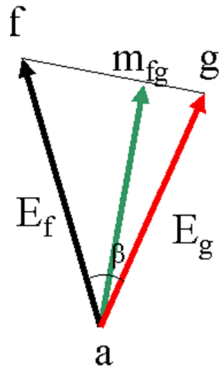
Figure 74: Forecasts f and g , either from two different NWP systems or from the same, but with different lead times, verifying at the same time. The errors E_f=(f-a) and E_g=(g-a) correlate cosine ( \beta ). Weighted together they yield a forecast m_{fg} with a RMSE which is lower than the errors E_f and E_g of the two averaged forecasts. The smaller the \beta , the larger their error correlation and the less m_{fg} will yield an error reduction.
