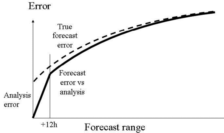
Figure 65: Forecasts verified against analyses often display a “kink” for the first forecast interval. This is because the error curve starts from the origin, where the forecast at t=0 is identical to the analysis. However, the true forecast error (forecasts vs. correct observations) at initial time ( t=0 ) represents the analysis error and is rarely zero. The true error curve with respect to the correct observations lies at a slightly higher level than the error curve with respect to the analysis, in particular initially.
