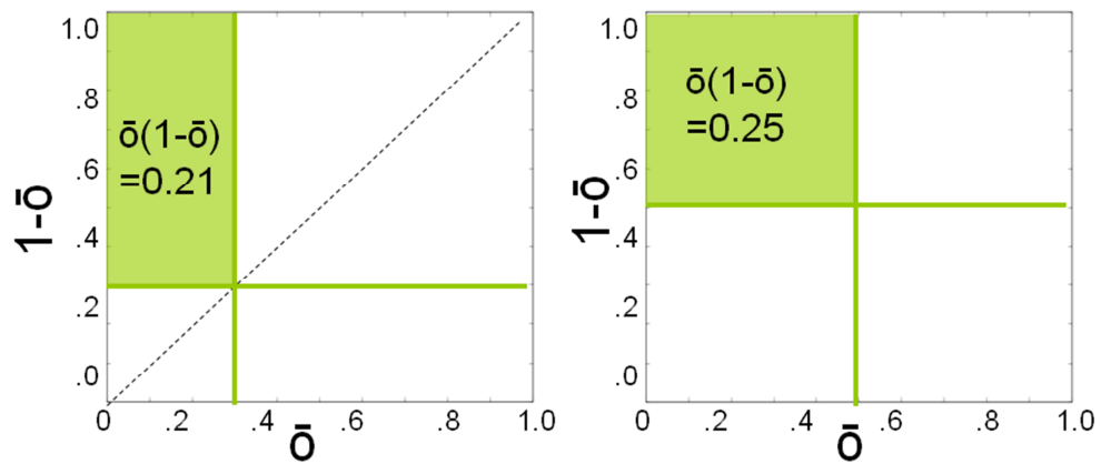
Figure 88: Uncertainty is at its maximum for a climatological observed probability average of 50%.
