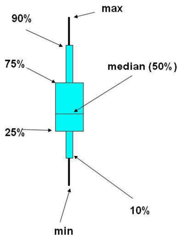
Figure 45: The box and whisker plot used in the ECMWF 10- and 15-day EPSgrams
