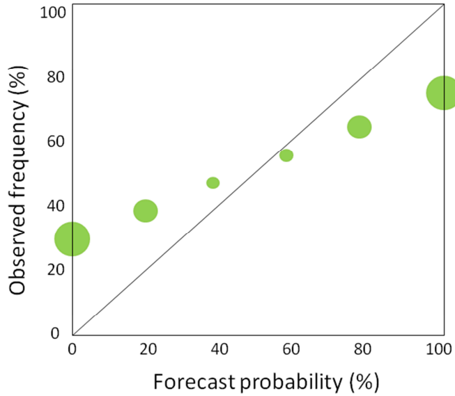
Figure 84: Probability forecasts with good sharpness but overconfident, since 0% forecasts are not always followed by dry weather, 100% forecasts not always followed by rain.
