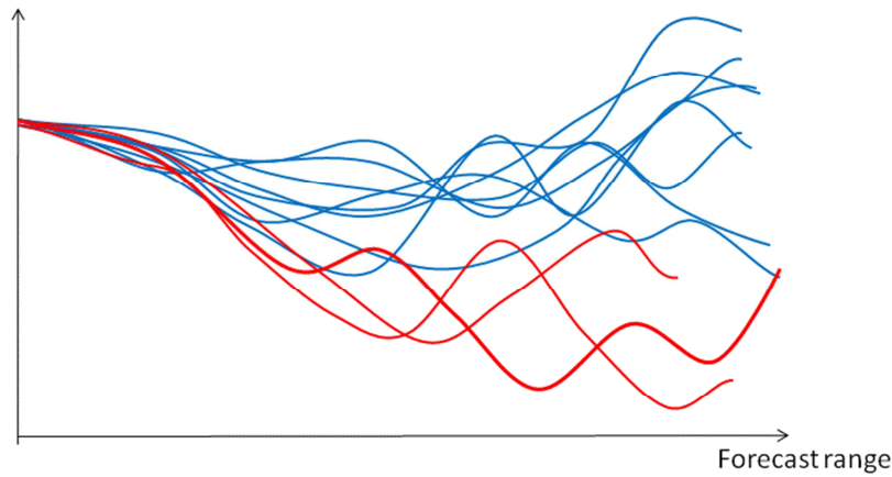
Figure 39: Same as Figure 36, for the case when the latest deterministic forecasts are not contained in the EPS ensemble
