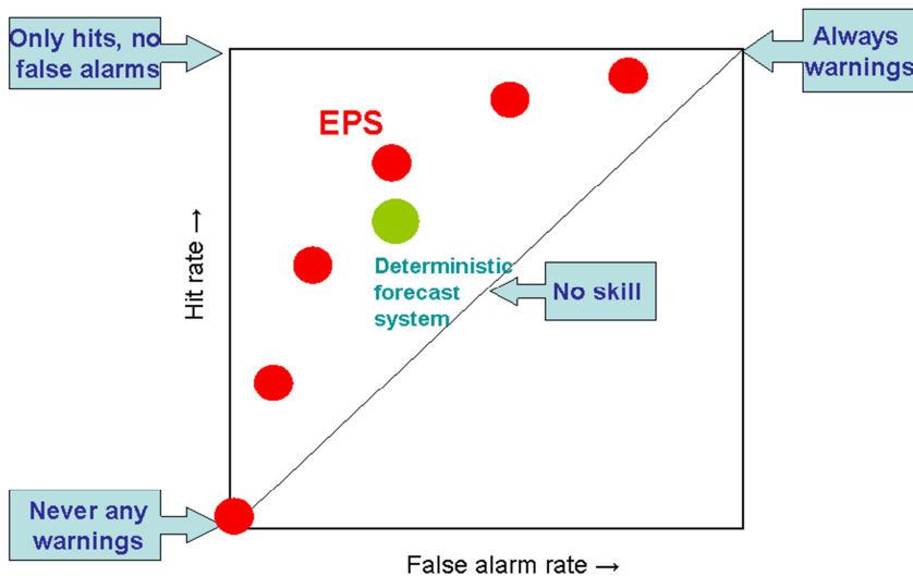
Figure 90: The same as above, but repeated for several thresholds between 0 and 100%, including the hit rates and false alarm rates of the deterministic model; although not providing probabilistic predictions it can be represented on the diagram by its typical hit rate and false alarm rate (green filled circle).
