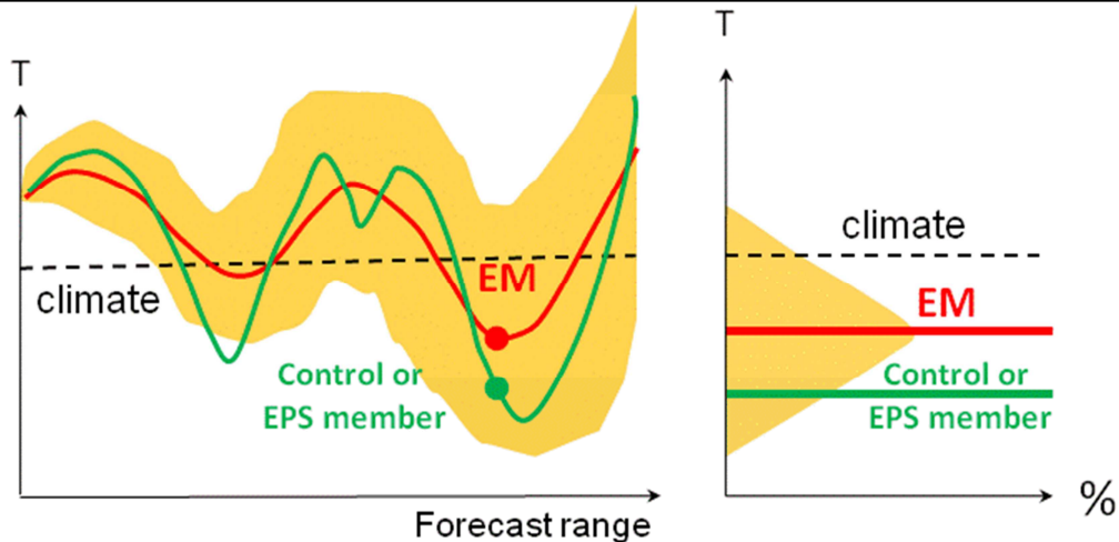
Figure 29: The diagram to the left shows schematically the relation between the spread of the ensemble for the whole forecast range (orange shaded area) and for two different types of deterministic forecasts. The EM (red line) lies in the middle of the ensemble spread whereas any individual ensemble member (green line), can oscillate within the ensemble spread. The Control, which does not constitute a part of the plume, can even on rare occasions (theoretically on average 4% of the time) be outside the plume.
