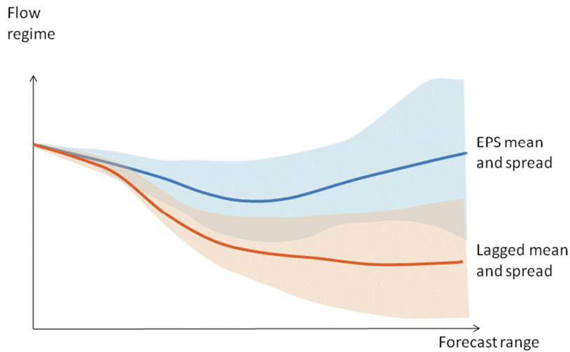
Figure 41: A schematic illustration of the combination of two ensemble forecasts with different EM (full lines).
