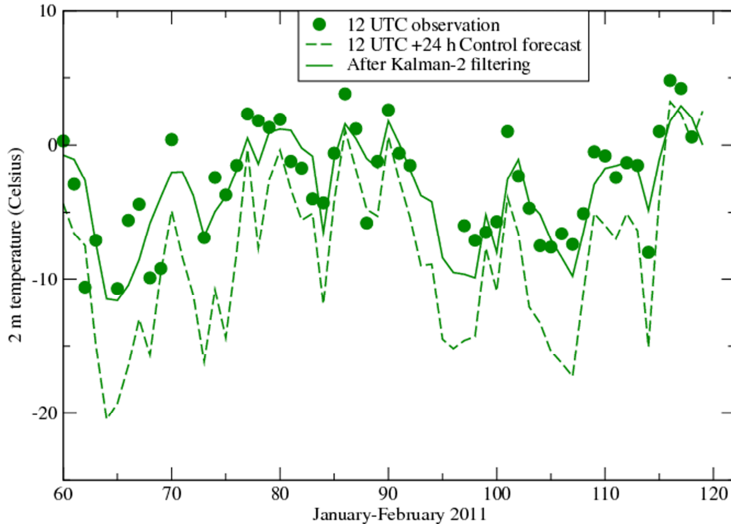
Figure 95: Adaptive Kalman filtering of 2-metre temperature forecasts for Tromsø in northern Norway during winter 2011. The forecasts are too cold and over-variable, both of which are remedied by X_1 and X_2 in a 2-parameter error equation.
