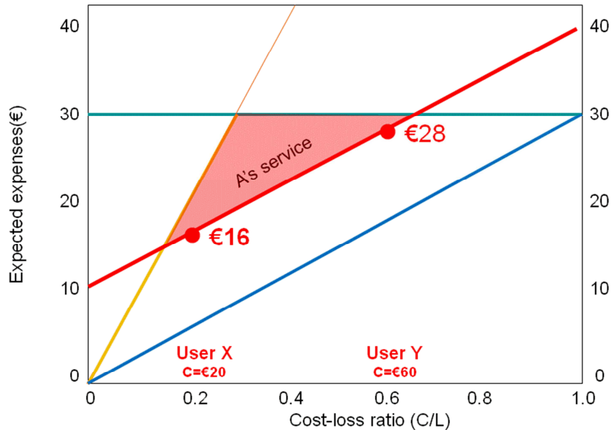
Figure 77: The same as above, but with the expected expenses for end-users served by forecast service A. The red area indicates the added benefits for X and Y from basing their decisions on deterministic weather forecasts from service A.
