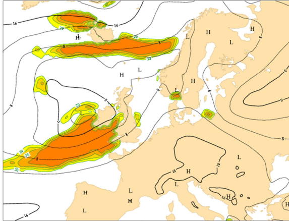
Figure 33: 1000 hPa EM 19 August 12 UTC +12 h valid at 20 August 00 UTC may serve as a proxy verification because of the small forecast range and the fact that the EM, thanks to the initial anti-symmetric nature of the perturbations, is almost identical to the Control. The probabilities essentially show where the verifying wind speed was > 10 m/s.
