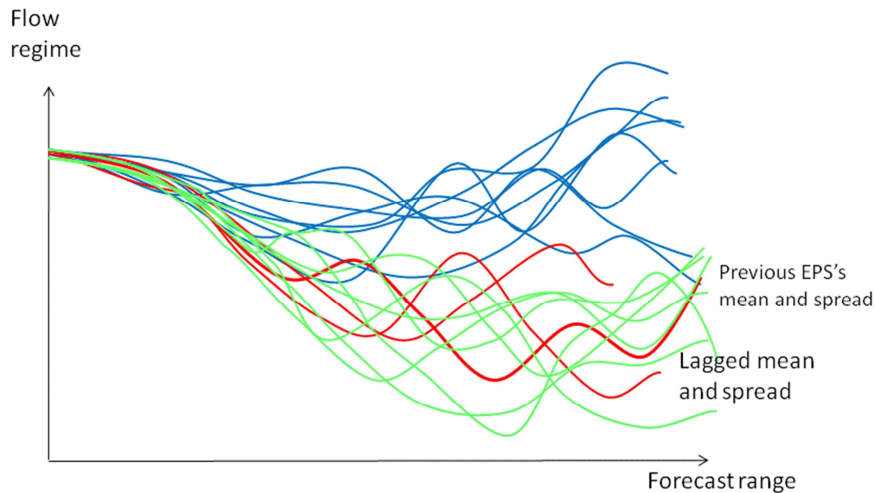
Figure 42: A schematic illustration of a case where the previous EPS (green lines) is in good agreement with the latest operational forecasts (red lines).
