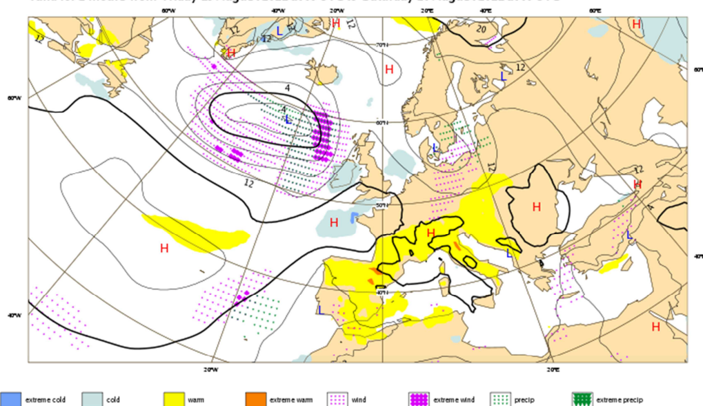
Figure 54: The global “anomalous weather” or “interactive EFI” chart from 17 August 2011, 00 UTC between +48 and +72 hours. It shows the geographical distribution of the EFI of the principal weather parameters: maximum wind gust, 24 h precipitation and 2 m temperature, overlaid with the ensemble mean of the 1000 hPa Z field.
