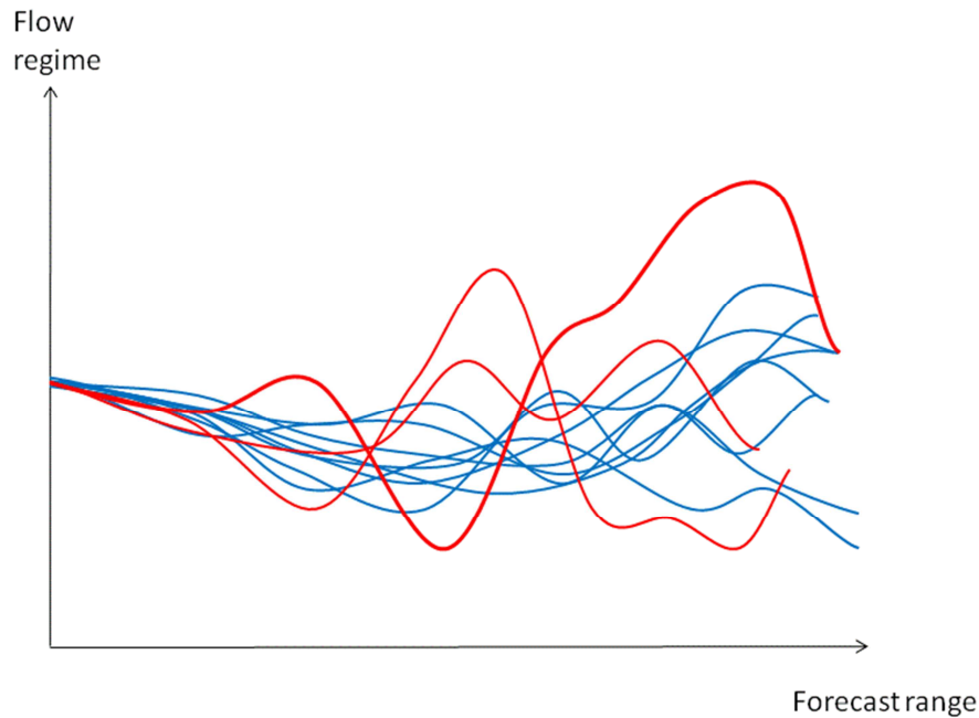
Figure 38: Same as Figure 36 for the situation with large forecast “jumpiness”, in spite of small ensemble spread.
