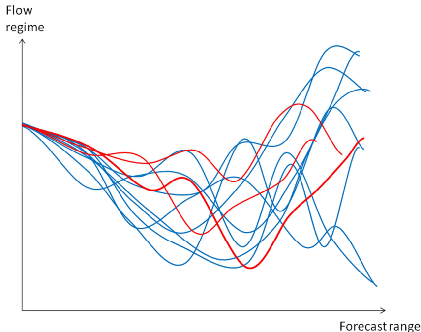
Figure 36: Schematic illustration of the relation between the ensemble forecasts (blue lines) and the latest deterministic forecasts (red lines) for the common case of general agreement. Since the order in which the forecasts have arrived might be significant, the thick, longest red line denotes the latest deterministic forecast, the thinnest, shortest red line the earliest.
