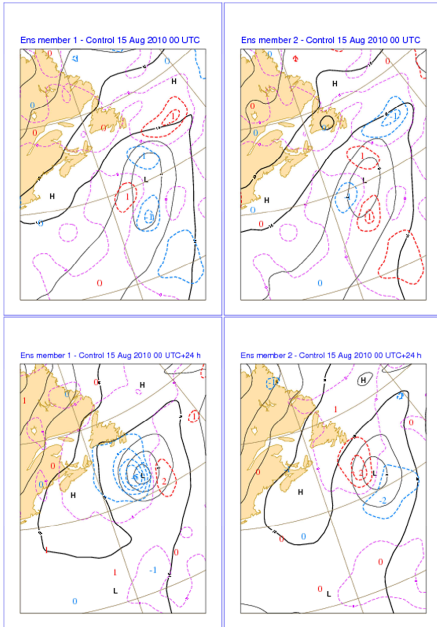
Figure 23: Same as Figure 22 but for 15 August 2010 00 UTC. In this case the antisymmetry is still clearly seen 24 hours into the forecast, member 1 having the low deepened and displaced into a slightly more westerly position, member 2 having the low weakened and displaced into a slightly more easterly position.
