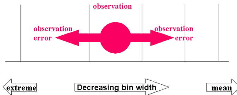
Figure 86: An observation (a filled circle) and its uncertainty assumed symmetric (the arrows). Since the forecast bins widen their intervals away from the centre (the mean of the distribution), an observation is more likely, for random reasons, to fall into an outer and wider bin than an inner and narrower one.
