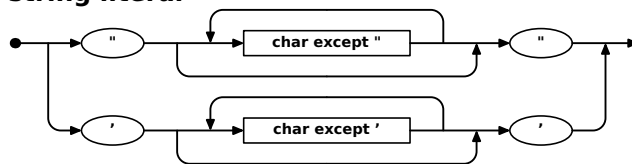
Figur 2.27: Jernbanediagram for (string literal)
