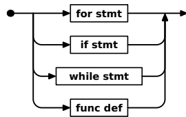
Figur 2.8: Jernbandediagram for <compound stmt>
