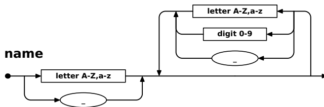
Figur 2.29: Jernbanediagram for (name)
