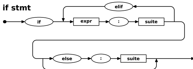
Figur 2.9: Jernbandediagram for <if stmt>
