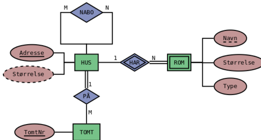
Figure 1: ER-modell
