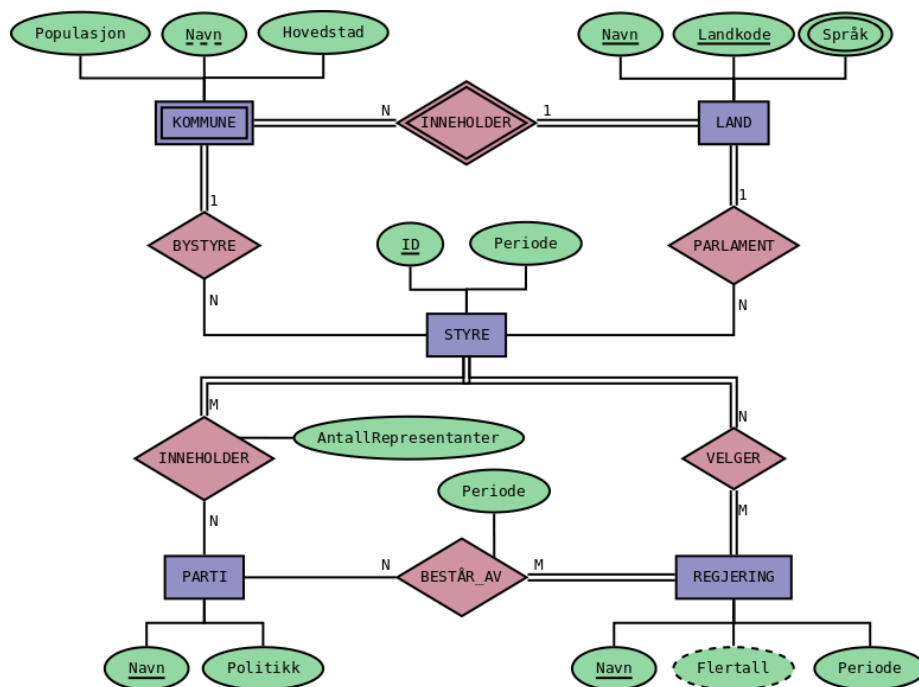
Figure 2: ER-modell over styrever
