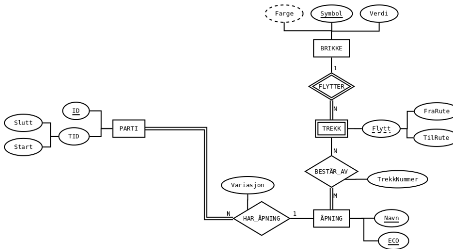
Figure 2: ER-modell
