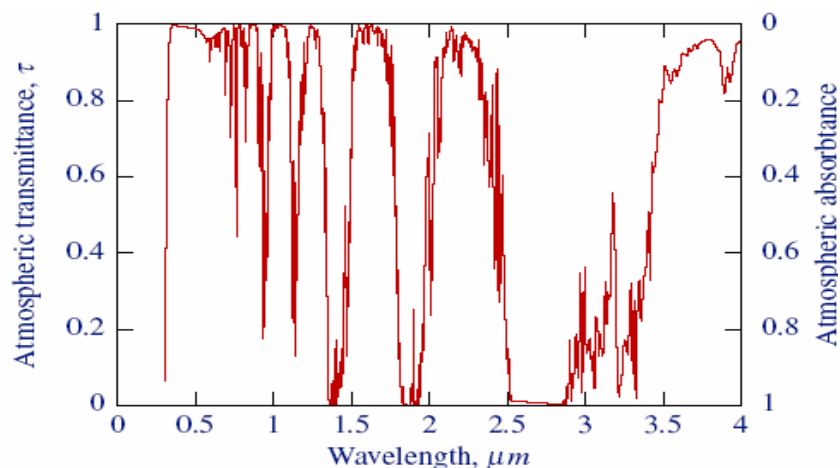
Figure 1-4. Atmospheric transmittance (left) and corresponding absorbance (right).
