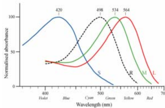
Figure 1-7. Normalized light sensitivity curves for retinal cones (S, M, L) and rods (R).
