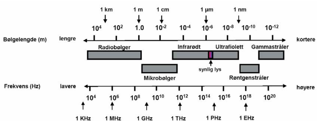
Figure 1-2. Wavelengths and frequencies for different parts of the spectrum.
