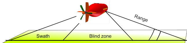
FIG. 29 Sidescan sonar geometry.
