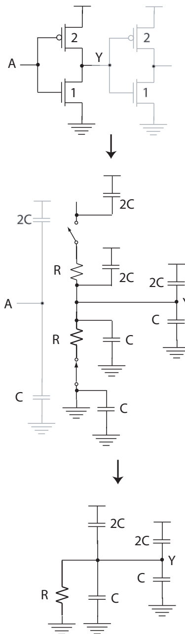
Fig. 11. Ekvivalent RC krets for en inverter. (FIG3.6)
