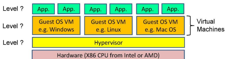
Type 1 VM Architecture (full virtualization)
