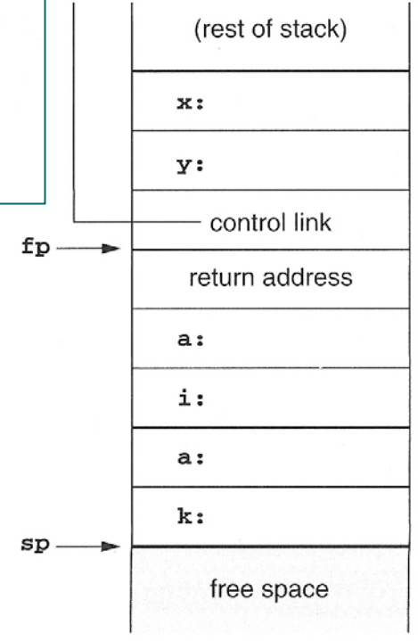
Activation record of call to P
