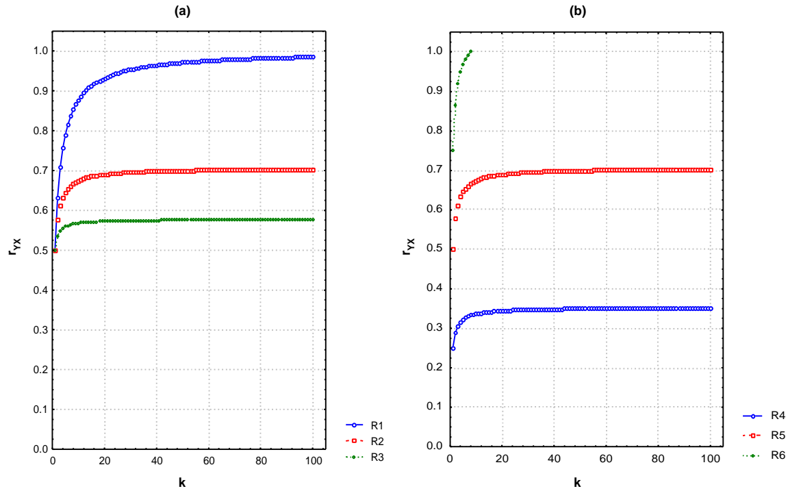
Figure 2: The two above panels show the behavior of the predictive validity coefficient as a function of the number of components in the X composite ( k ) as it varies up to 100. The plots in panel (a) are for \bar{r}_{YX} fixed at 0.5, and \bar{r}_{xx} varies as follows: plot R1 is for \bar{r}_{xx}=0.25 , plot R2 is for \bar{r}_{xx}=0.5 , plot R3 is for \bar{r}_{xx}=0.75 . The plots in panel (b) are for \bar{r}_{YX} fixed at 0.5, and \bar{r}_{xx} varies as follows: plot R4 is for \bar{r}_{xx}=0.25 , plot R5 is for \bar{r}_{xx}=0.5 , plot R6 is for \bar{r}_{xx}=0.75 .
