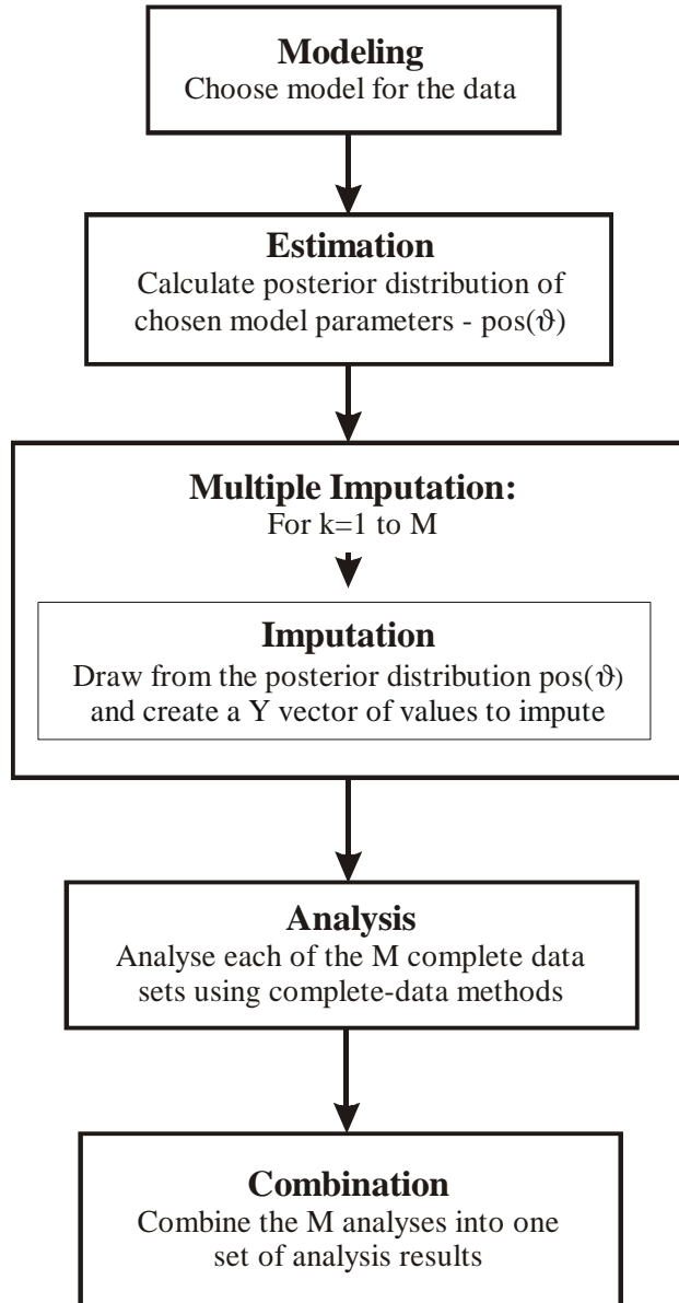
Figure 10: Schematic showing the tasks involved in multiple imputation.
