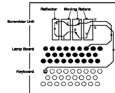
http://www.math.miami.edu/~harald/enigma/enigma.gif
