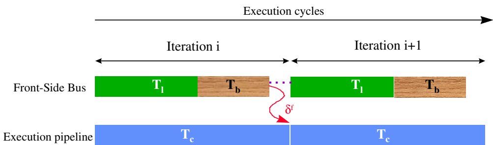
Figure E-3 Compute Bound Execution Pipeline
