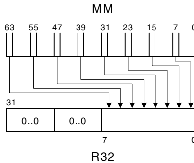
Figure 4-7 pmovmskb Instruction Example
