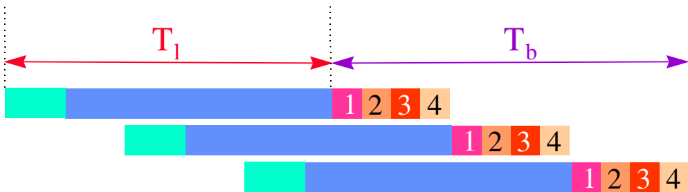
Figure E-1 Pentium II, Pentium III and Pentium 4 Processors Memory Pipeline Sketch
