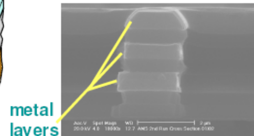
M1-2-3 with field oxide
