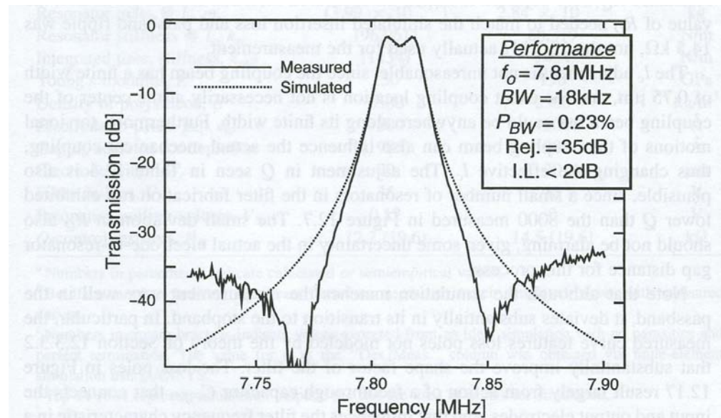
Figure 12.17. Measured spectrum for a terminated 7.81 MHz \mu mechanical filter with excessive input/output shunt capacitance. Here, Q_{\text{filtr}} = 435 . (From reference [18])
