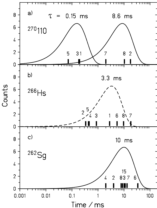
Fig. 2. Time distribution of the subsequent \alpha -decays (a,b) and fission events (c) measured in the reaction ^{64}\text{Ni} + ^{207}\text{Pb} . The curves represent the density distribution (arbitrary ordinate scale) of counts in a radioactive decay on a logarithmic time scale with logarithmically increasing channel width [4]. The position of the curve determines the lifetime, it was adjusted to the data by a least-squares analysis. The dashed curve in plot b) indicates that the data are also compatible with two lifetimes of 0.5 and 9 ms (see text). The numbers from 1 to 8 assign the events to the measured decay chains.
