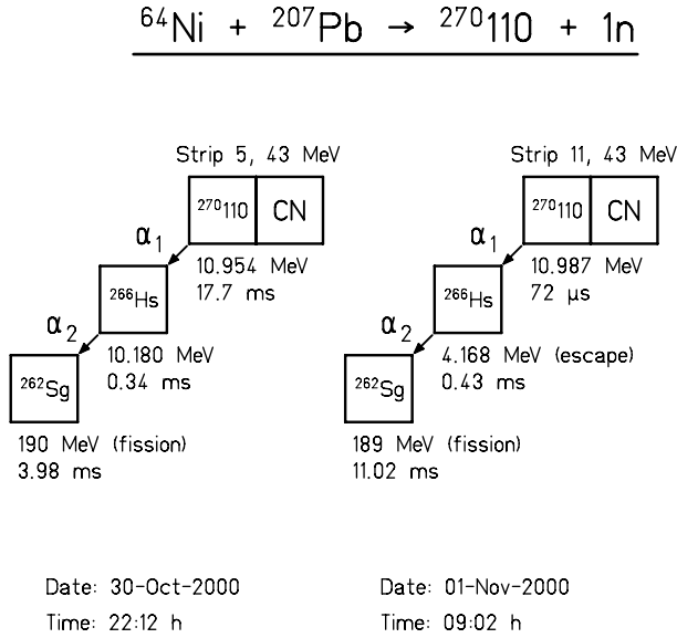
Fig. 1. Two representative decay chains observed in irradiation of a {}^{207}\text{Pb} target with {}^{64}\text{Ni} projectiles. The chain on the left side starts with a relatively long-lived \alpha -decay of {}^{270}\text{110} which is attributed to a high-spin K isomer. The chain on the right side represents the decay of the short-lived ground state.
