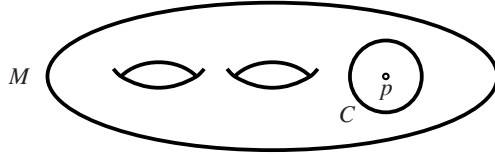
Fig. 28.3. Punctured surface.
