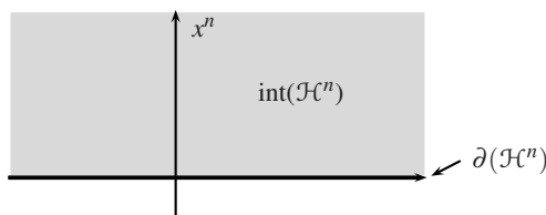
Fig. 22.1. Upper half-space.
