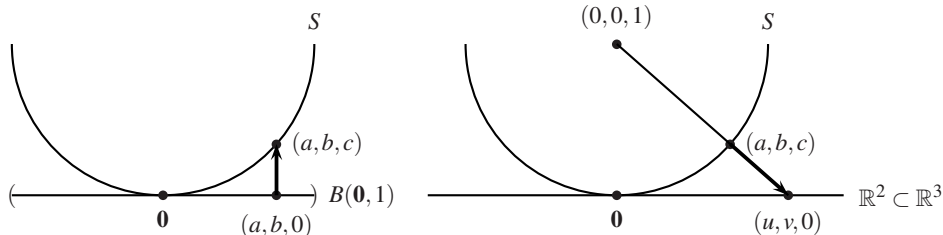
Fig. 1.4. A diffeomorphism of an open disk with \mathbb{R}^2 .
