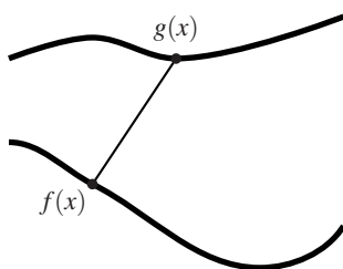
Fig. 27.1. Straight-line homotopies.
