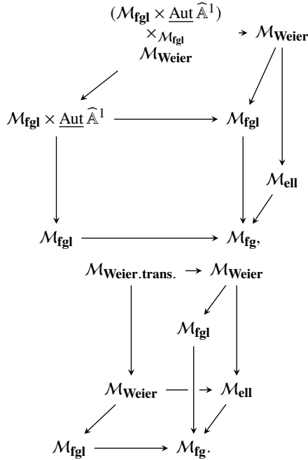
Figure A.1 Two expressions of the same cubical pullback.
