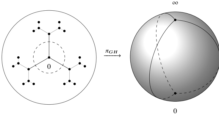
Figure 4.5 The period map at n = 2 , p = 2
