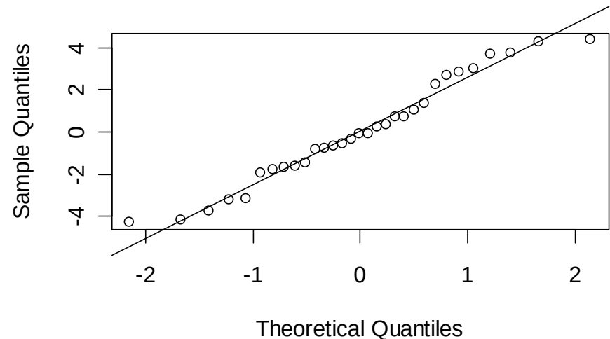
Q-Q plot
